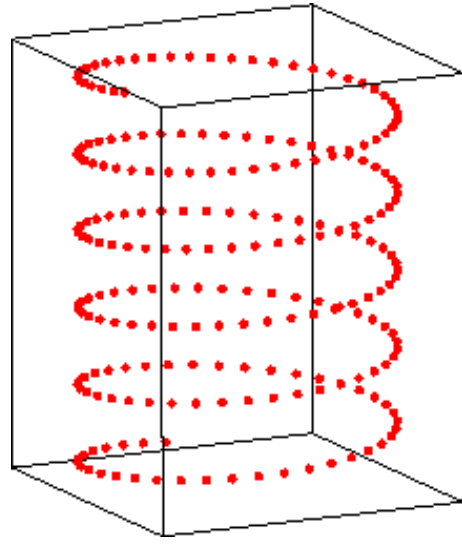
Figure 1: No radiative energy loss: |\partial_{\vec{z}} \vec{M}^T| = 1
