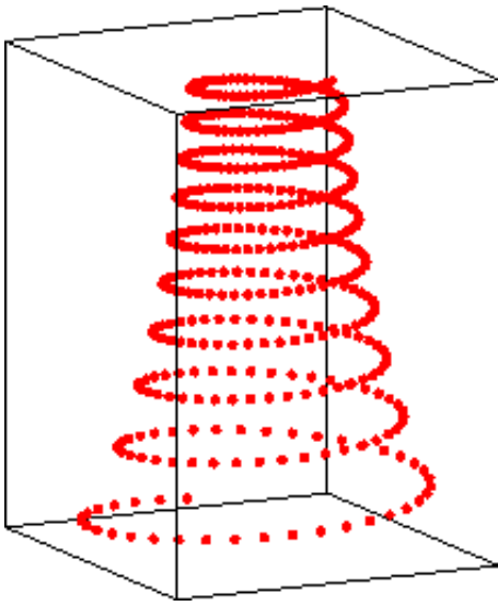
Figure 2: With radiative energy loss: |\partial_z \vec{M}^T| = 0.023
