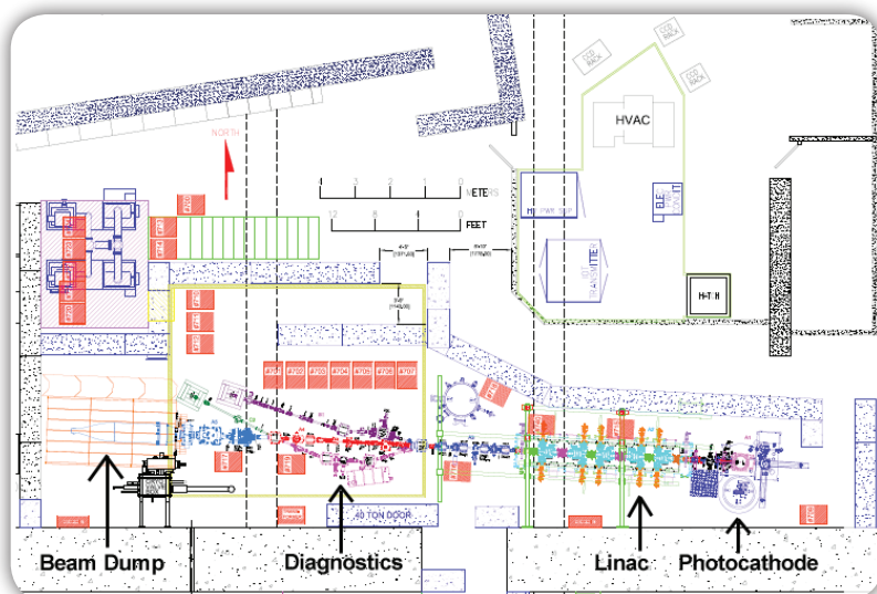
Fig. 1: Floor layout of the ERL test area in L0 of Wilson Laboratory, just south of CHESS East. From right to left: DC photocathode, superconducting linac, branch lines for diagnostics, and finally, a high power beam dump.
