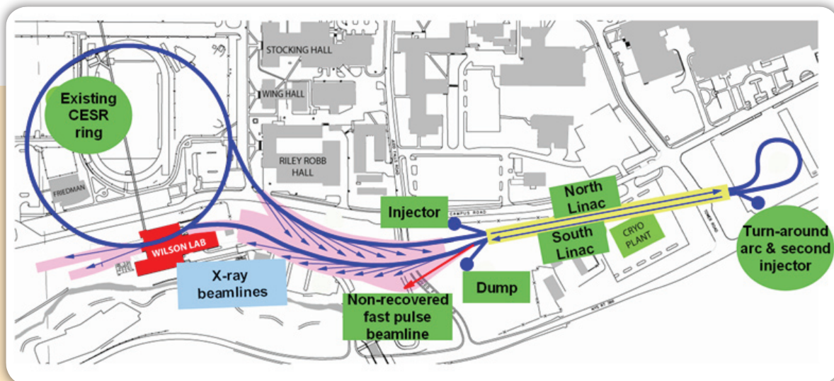
Fig 5: Low-energy electrons are made and accelerated to 5-10 MeV at the injector. They are raised to 2.5 GeV in the North Linac by traveling “on-crest” through the RF fields produced by the SRF cavities, turned around and raised to 5 GeV after passing through the South Linac. X-rays will be produced in undulators in the position of the blue arrows, mostly in a new building to be added to the east of Wilson laboratory. Electrons returning to the North Linac are shifted 180 degrees out of accelerating phase (by adjusting the path length) so that the electrons are now “off-crest” and their energy is recovered in both linacs before the spent electron beam is sent to the dump. There is room in the layout for a non-energy-recovered, fast-pulse beamline as shown by the red arrow.
