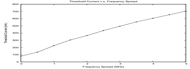
Figure 4: The threshold current v.s. Frequency spread
