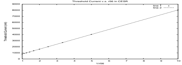
Figure 3: Threshold Current v.s. 1/r_{56}
