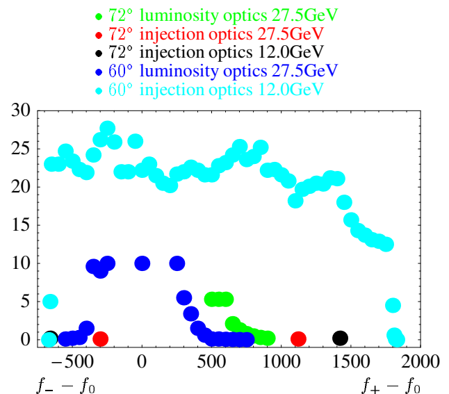
Figure 1: Lifetime (in hours) as a function of rf frequency shift \Delta f for four different machine settings.
