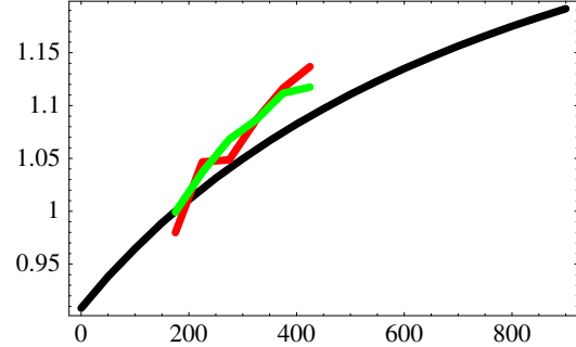
Figure 3: Relative increase of luminosity with increasing rf frequency for ZEUS (red), H1 (green), and simulated (black). If the simulation would assume f_0 to be 175 Hz below f_c , the curve would shift to the left leading to good agreement with the measurement.
