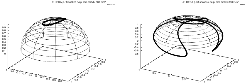
FIGURE 1. The field \hat{n} in HERA- p calculated with SPRINT on the 4\pi mm mrad (left) and the 64\pi mm mrad (right) ellipses at 800 GeV. A normalised emittance of 4\pi mm mrad \equiv “ 1 - \sigma ”.
