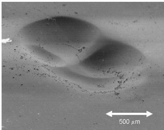
Figure 3: Pit defect found at quench location in a single cell cavity. The bar is 500 microns.
