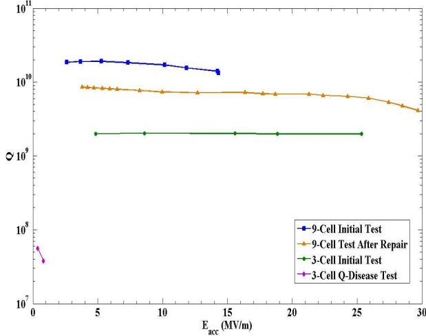
Figure 4: RF performance of the two multi-cell reentrant cavities fabricated in a joint effort between AES and Cornell University. Four RF performance curves are shown: 1) the 9-cell cavity at 2.0 K limited by a pit-defect, 2) the 9-cell cavity at 1.7 K after tumbling-repair of pit-defect, 3) the 3-cell cavity after its first cooldown at 1.6 K, and 4) the 3-cell cavity after a warm-up to 100°C-135°C for 30 hours and a rapid cool to 1.6 K.
