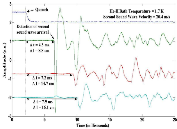
Figure 1: A quench event. Four traces are shown: 1) the upper trace is the quenching-cavity transmitted power, 2-4) the lower traces are transducer second sound signals.
