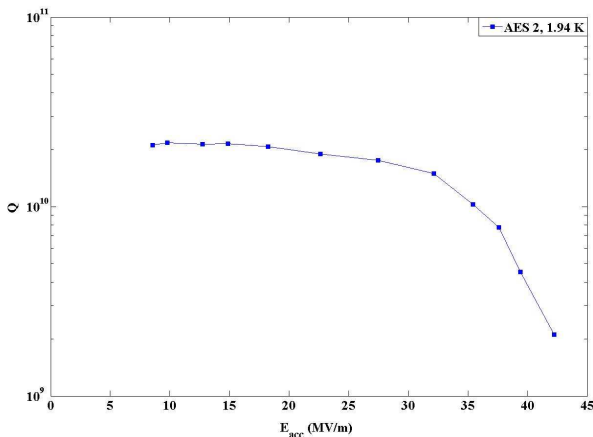
Figure 6: AES cavity 1.94 K performance after vertical electropolishing and hydrogen degassing. The cavity started field emitting at 22 MV/m and never quenched.
