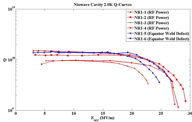
Figure 5: Q-curves for the six Niowave Inc. single-cell cavities tested at Cornell. All cavities exhibited the high-field Q-slope common to BCP cavities and two cavities quenched at equator weld defects.
