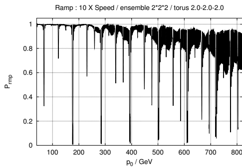
Figure 1: The polarisation during acceleration to 803 GeV for 2\sigma in all 3 phase space amplitudes for the snake layout of figure 2.
