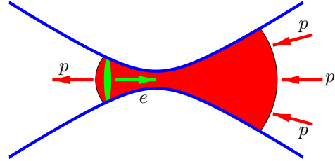
Figure 1: The bunch size changes during the collision due to the hourglass effect.
