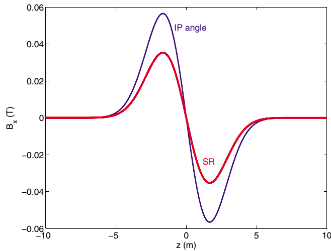
FIG. 6. (Color) Horizontal field of the detector integrated dipole (DID) for the SiD detector. The DID strength is optimized to zero the IP vertical angle (blue line) or to minimize the SR vertical beam size growth (red line) in the case of bare SiD without antisolenoids.
