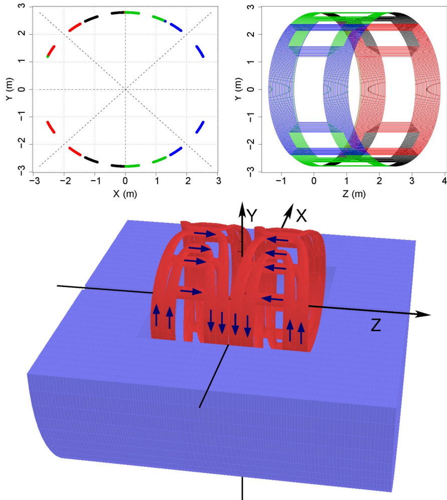
FIG. 10. (Color) Detector integrated dipole corrector. The top plot shows the actual arrangement of windings in one half of the corrector. The second half of the corrector is mirror symmetrical with respect to the solenoid center ( z = 0 ). The bottom plot shows a simplified model used for 3D field calculations with TOSCA (OPERA3D code) to evaluate the effect of iron in the SiD yoke on the dipole field. For ease in viewing the 3D model the solenoid coil and the top half of the SiD yoke are not shown. The arrows show the direction of the current. Except for a small deviation near the start of the end cap around Z = \pm 3.2 m the horizontal field profile is very close to that assumed for the tracking studies shown in Fig. 6.
