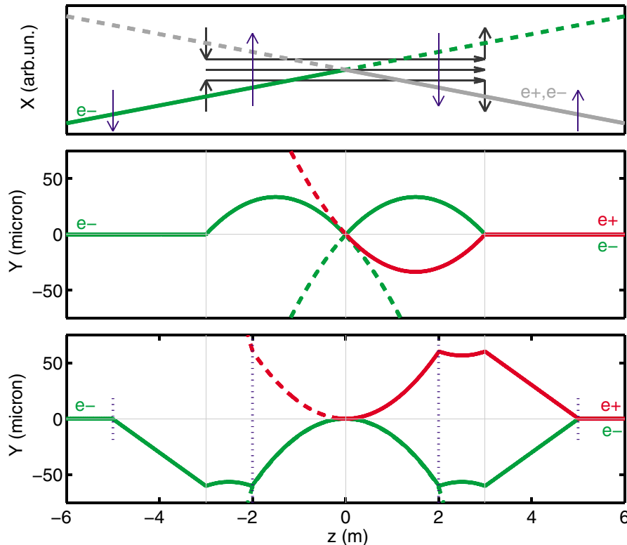
FIG. 1. (Color) Illustration of e^+e^- and e^-e^- collisions in a detector solenoid field with sharp edges (schematically shown in the top plot) without (middle) and with (bottom) compensation of the IP angle by the detector integrated dipole and two external correctors. The model parameters are L = 3 m, \theta_c = 10 mrad, B_0 = 5 T, beam energy 250 GeV. The uncompensated vertical angle at the IP is approximately 45 \mu\text{rad} . The compensation kicks are shown on the top plot by the blue arrows; they are located at z = \pm 2 m and z = \pm 5 m and their magnitudes are 75 and 30 \mu\text{rad} . The IP is at z = 0 m. Outgoing beams are shown by thick dashed curves.
