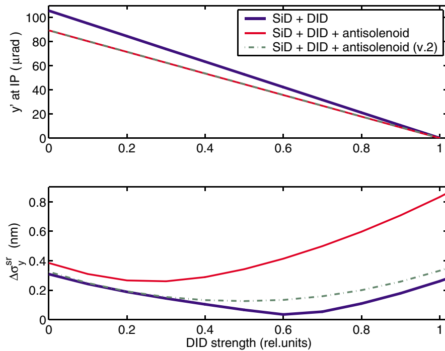
FIG. 9. (Color) Vertical angle at the IP (top) and the beam size growth due to synchrotron radiation (bottom), versus strength of the DID corrector, without antisolenoid (thick blue line), with the antisolenoid with parameters suggested in [1] (red line), and with the antisolenoid optimized to reduce the SR effects (green dash-dotted line).
