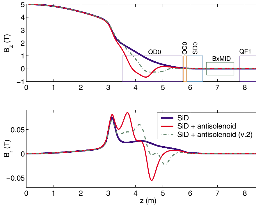
FIG. 3. (Color) Longitudinal and radial magnetic field in SiD calculated by ANSYS, without and with the weak antisolenoid which cancels the beam distortions produced by the detector solenoid. The red line shows the field with the antisolenoid parameters suggested in [1], and the green dot-dashed line shows the field with another configuration of the antisolenoids, optimized to reduce SR effects (see text). The radial field is at the nominal beam trajectory with half crossing angle \theta_c = 10 mrad. Locations of the final doublet elements (quadrupoles QD0 and QF1, sextupole SD0, octupole OC0, and an optional dipole corrector BxMID) are also shown. The IP is at z = 0 m.
