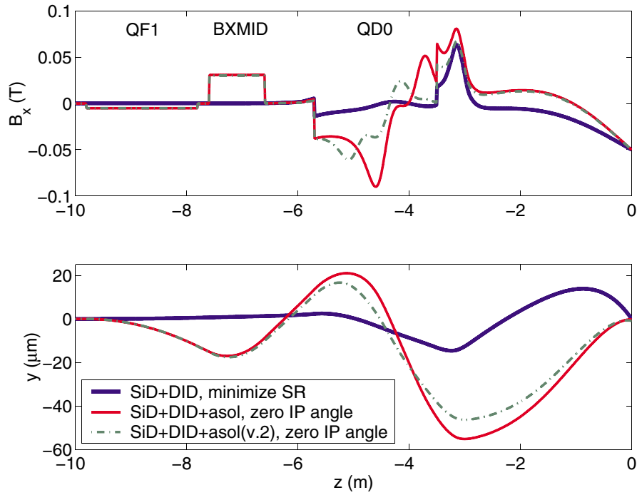
FIG. 8. (Color) Horizontal field on the beam axis (top) and beam orbit determined by tracking (bottom) in three cases: (i) bare SiD (no antisolenoid) and DID strength optimized to minimize SR beam size growth (blue thick line), \Delta\sigma_y^{SR} = 0.034 nm; (ii) SiD with antisolenoid (parameters from [1]) (red line), \Delta\sigma_y^{SR} = 0.83 nm; (iii) SiD with antisolenoid optimized to minimize SR effects (green dash-dotted line), \Delta\sigma_y^{SR} = 0.33 nm. In the last two cases the IP angle is compensated by the DID, FD offsets, and BXMID without introducing any linear or second order dispersion.
