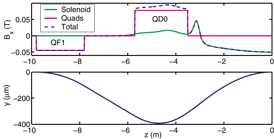
FIG. 5. (Color) Illustration of IP angle compensation using only offsets of the final doublet quadrupoles. Horizontal field on the beam axis (top), beam orbit calculated by tracking (bottom). Contributions of the solenoid and FD quadrupoles are shown on the top plot separately. The beam size growth due to synchrotron radiation is \Delta\sigma_y^{\text{SR}} = 5.2 \text{ nm} .
