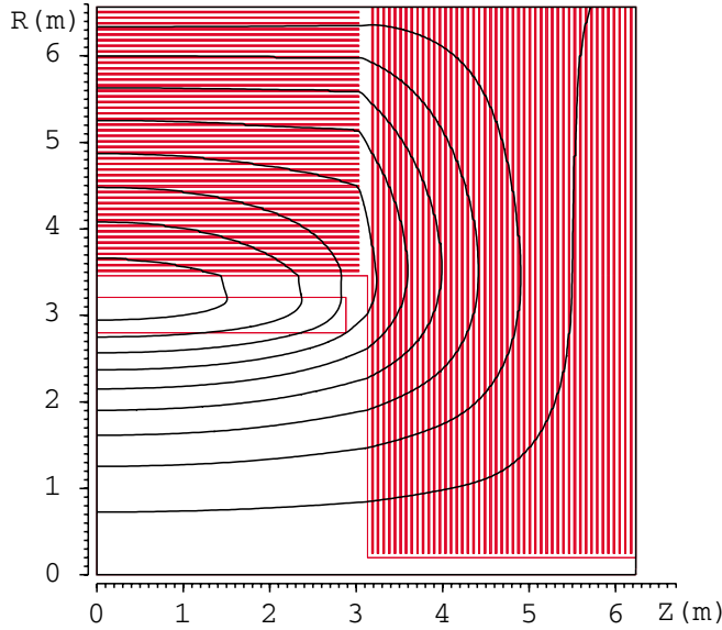
FIG. 2. (Color) Schematic of the silicon detector (SiD) with magnetic field lines calculated by ANSYS. The IP is at z = 0 m.
