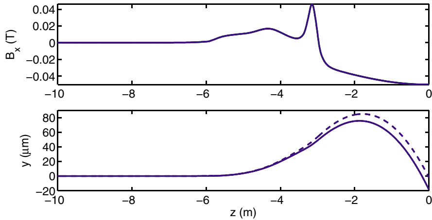
FIG. 4. (Color) Horizontal field strength on the beam axis of the SiD detector (top), and vertical beam orbits (bottom), in the absence of vertical IP angle compensation. The orbit calculated in the absence of any focusing elements is shown by a dashed line, and the orbit determined by tracking with DIMAD is shown by a solid line on the bottom plot. For the tracked beam, the IP beam coordinates are x = 0.65 \mu\text{m} , y = -18.5 \mu\text{m} , x' = -0.21 \mu\text{rad} , and y' = -104 \mu\text{rad} . The beam size growth due to synchrotron radiation is \Delta\sigma_y^{\text{SR}} = 0.31 \text{ nm} .
