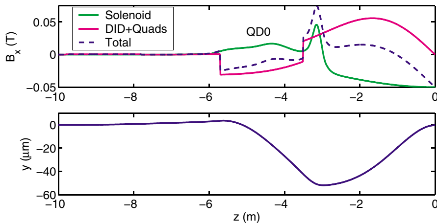
FIG. 7. (Color) Horizontal field on the beam axis (top) and the beam orbit (bottom). The IP angle has been compensated using DID and offsets of QD0 and QF1 quadrupoles. The orbit is determined by tracking. The beam size growth from synchrotron radiation is \Delta\sigma_y^{\text{SR}} = 0.26 \text{ nm} .
