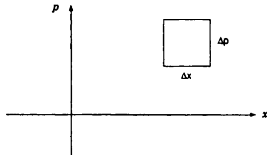
Figure 6.10. Infinitesimal area of phase space.
