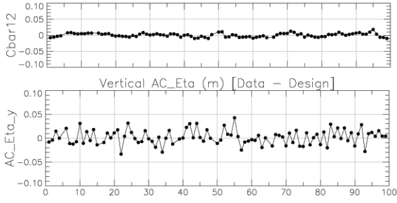
Figure 2: Measured coupling and vertical dispersion after low-emittance tuning. Horizontal axis is BPM index. RMS Cbar12 = 0.006 , RMS vertical dispersion = 15mm.
