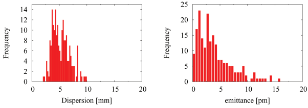
Figure 1: Vertical dispersion and emittance after low emittance tuning procedure for 200 machine configurations with alignment errors and measurement resolution described in the text.
