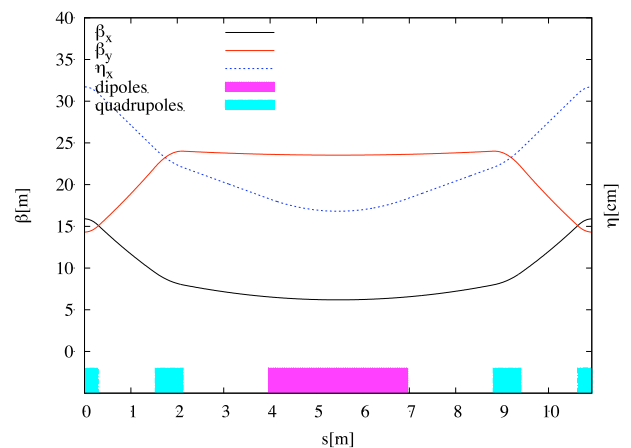
Fig. 1: Arc cell
