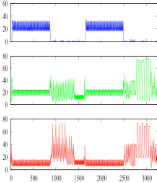
Fig. 2: Optical Functions. From left to right, arc, phase trombone, RF, wigglers, arc, circumference changing chicane, injection, extraction.
