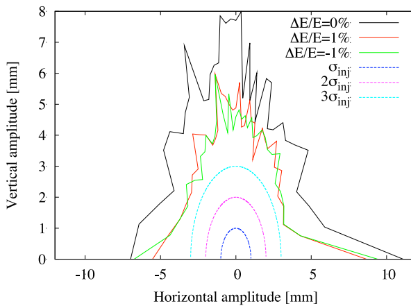
Fig. 3: Dynamic aperture.
