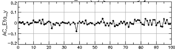
Figure 9: Measured vertical dispersion with no gain or tilt correction. Transverse coupling and vertical dispersion have been jointly minimized through an optimization of skew quadrupoles and vertical steerings. The residual dispersion is 20mm RMS.
