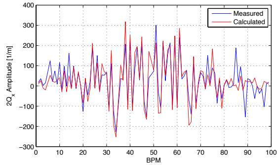
Figure 13: Amplitude of the in-phase response at 2Q_x . The blue line is the measurement and the red the model.
