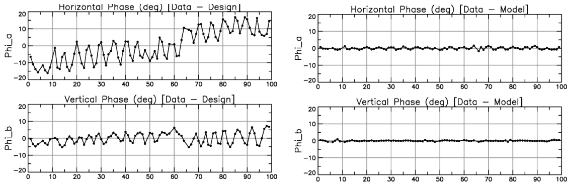
Figure 1: Vary the strengths of all quadrupoles in the lattice model until the model betatron phase matches the measured phase for the nominal K_1 of the quadrupole being calibrated. This is referred to as the “base fit”. Left : Difference between the measured horizontal and vertical betatron phase and the design values of the phase. Right : Difference between the measured and the fitted model values.
