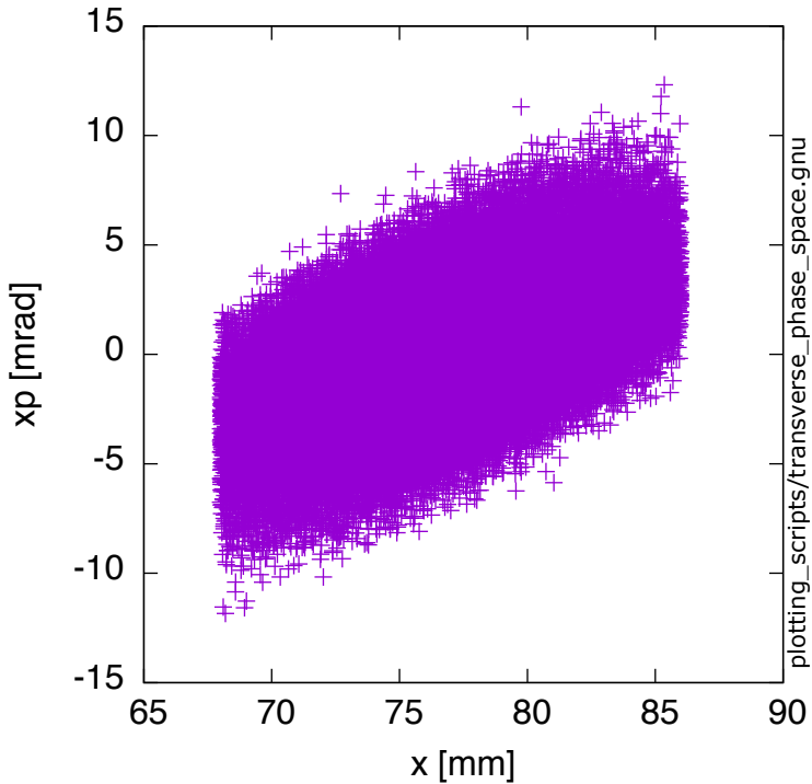
lost_muons-RING_BR_phase_space.dat
