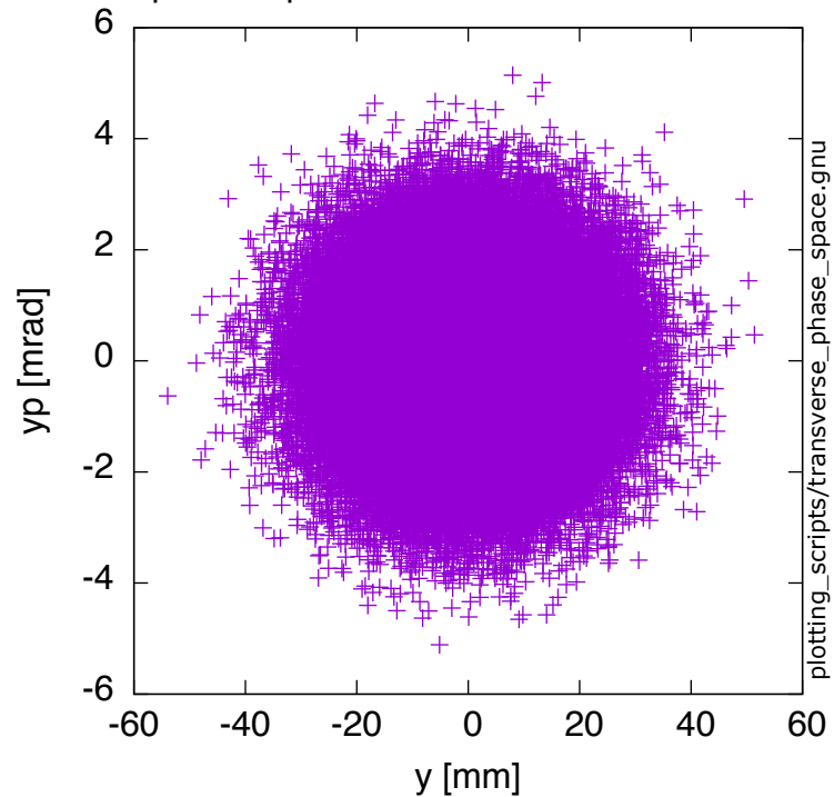
lost_muons-InflectorExitNoScatter_phase_space.dat
