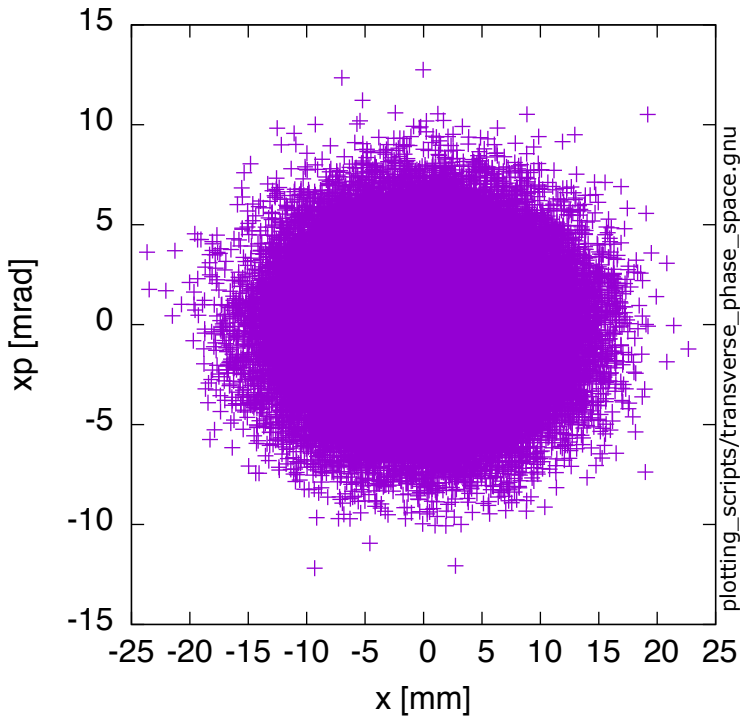
lost_muons-InflectorExitNoScatter_phase_space.dat
