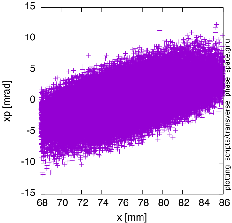
lost_muons-INJ_TO_RING_phase_space.dat
