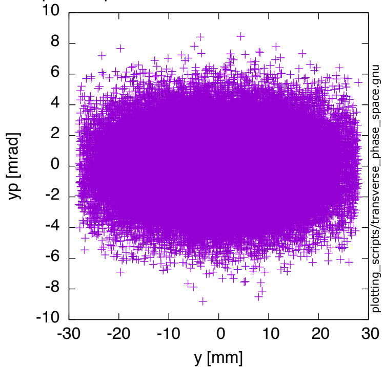
lost_muons-INJ_TO_RING_phase_space.dat
