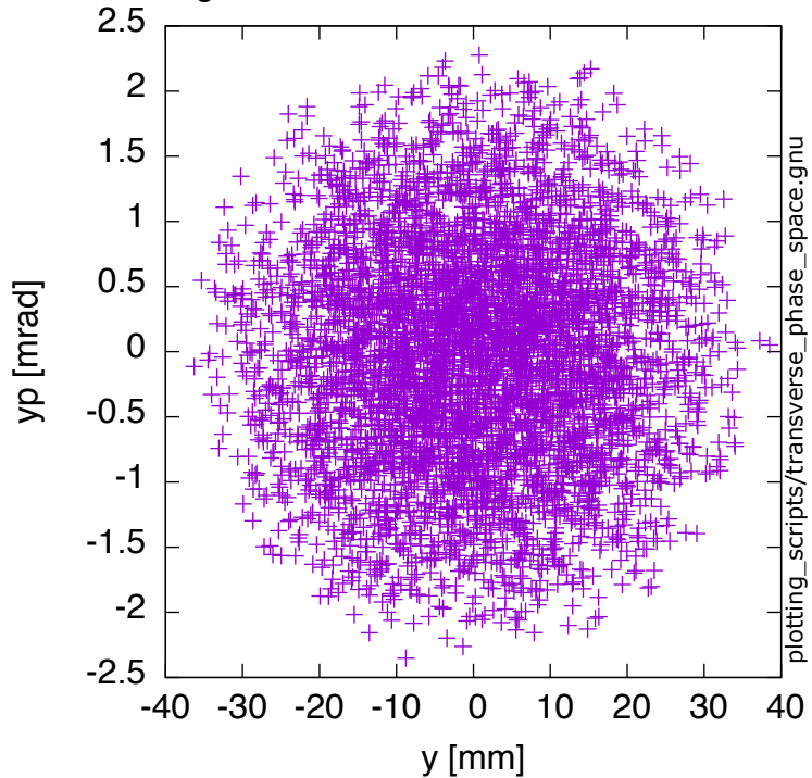
lost_muons-EndOfTracking
