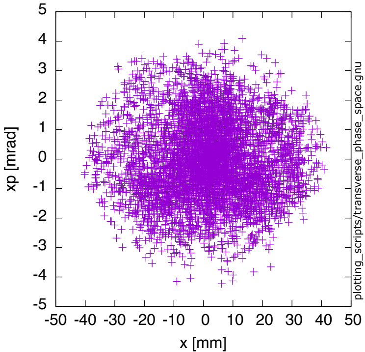
lost_muons-EndOfTracking
