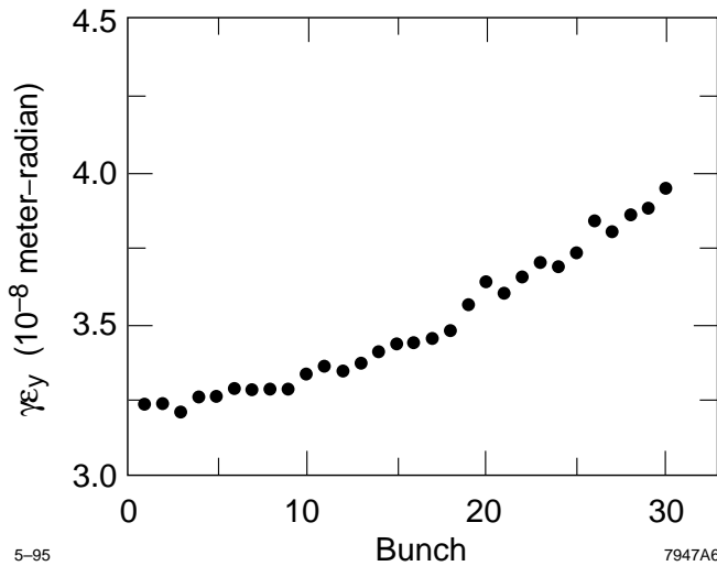
5-95 7947A6 Figure 3. Simulation of emittance correction in the NLC-I prelinac with a shortened bunch train of 30 bunches and a vacuum pressure of 3 \times 10^{-8} Torr of CO gas; because the ions are trapped, this is equivalent to a vacuum pressure of 1 \times 10^{-8} Torr and a train of 90 bunches.
