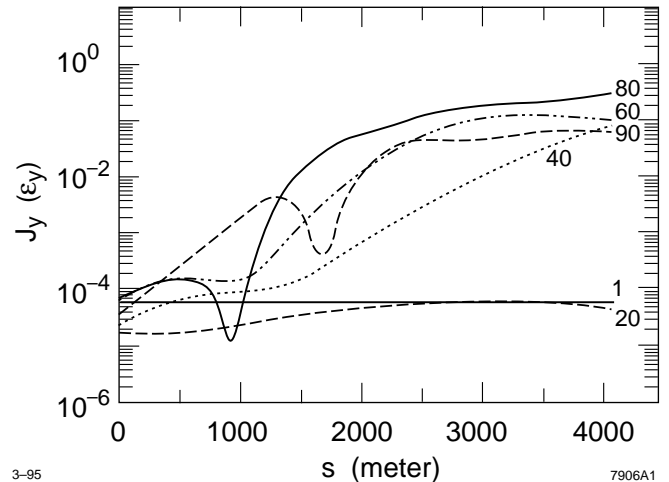
Figure 8. Growth of the action of the vertical centroid for every twentieth bunch in the NLC Damping Ring for a vacuum of 10^{-8} Torr of CO gas; note that the growth saturates at roughly \sigma_y because of the nonlinearity of the beam-ion force (from Ref. [18]).
