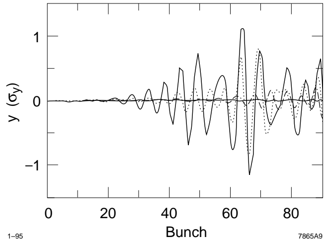
Figure 7. Position of vertical centroids along the electron bunch train after being stored for 0 \mu s (solid), 0.67 \mu s (dashes), 1.3 \mu s (dots), and 2 \mu s (solid) in the NLC Damping Ring with a vacuum of 10^{-7} Torr of CO gas; note that the modulation of the electrons goes to roughly \sigma_y after 2 \mu s (from Ref. [16]).
