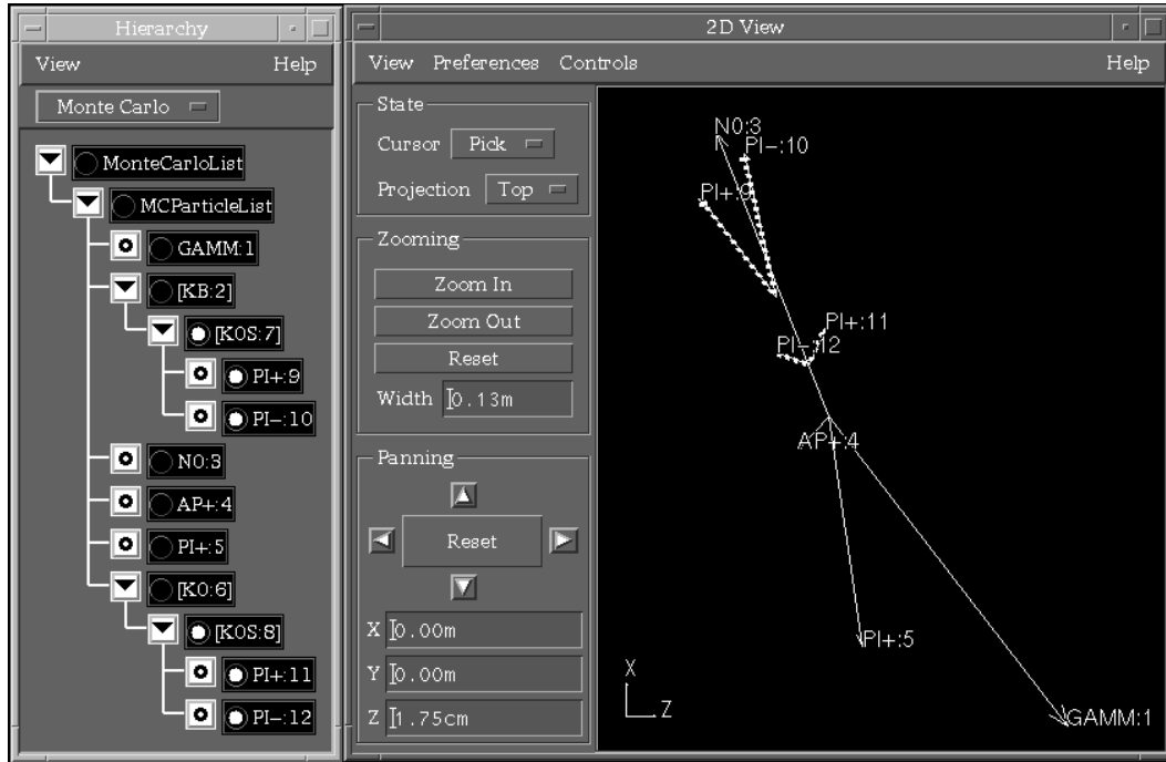
Fig. 1. Picture of the Hierarchy and 2D view both only showing Monte Carlo particles. The 2D view represents the Monte Carlo particles as vectors labeled with their names. To simplify the image, the kaons are invisible. The views show that the K_s^0 's and their daughters have been selected.
