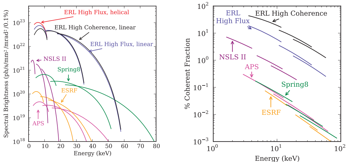
Figure 1.3.3: (Left) The average spectral brightness vs. energy for the 1) ERL in Hi-flux mode (5 GeV, 100 mA, 30 pm round beam, 22 mm period ID) and ERL in Hi-coherence mode (5 GeV, 25 mA, 8 pm round beam, 22 mm period ID). Even higher brightness may be feasible with advanced undulators or advanced beam collimation; 2) Spring8 (8 GeV, 100 mA, 3.4 nm \times 6.8 pm emittance, 3.2 cm period ID); 3) NSLS II (3 GeV, 500 mA, 0.55 nm \times 8 pm, 14 mm period SC Undulator); APS (7 GeV, 100 mA, 2.5 nm \times 20 pm, 3.3 cm ID). (Right) Coherent fractions for the various sources are indicated.
