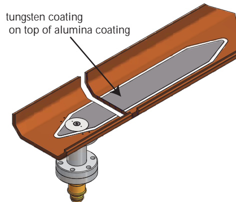
Figure 2.2.23: Electrode deposited on the vacuum chamber via thermal-spray technology. The electrode has already been used for electron clearing in a superconducting wiggler as a part of CEsrTA project.
