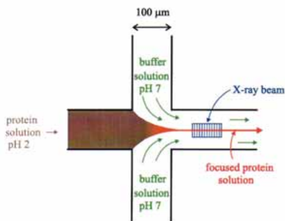
Figure 1.2.3: A micromixer utilizes diffusional equilibrium of the lamellar flow of a submicrometer wide jet between side-streams in a lithographically-fabricated mixer cell. Microsecond mixing times occur with submicron-wide jets.
