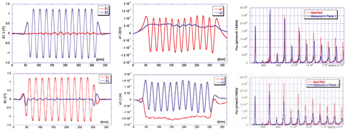
Figure 2.7.10: Measured magnetic field components (left), and predicted trajectories (center), and on-axis x-ray spectrum (right) in planar modes.
