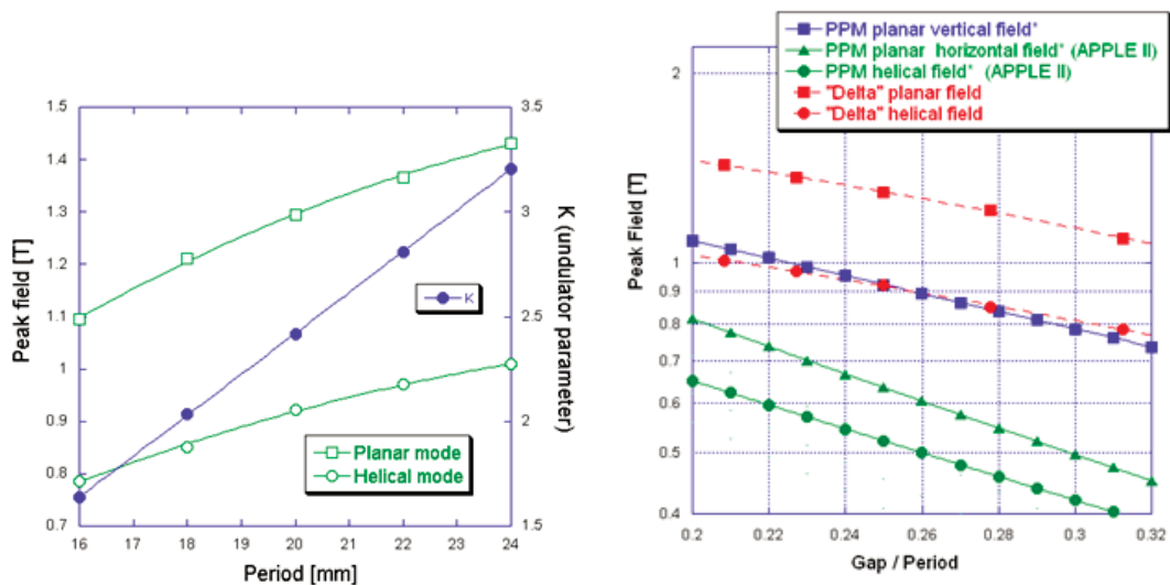
Figure 2.7.5: Left plot – peak field in planar and helical modes and undulator parameter K as a function of period. Right plot – peak field as function of gap over period ratio for ‘Delta’ and others PPM undulators.
