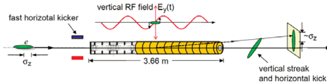
Figure 2.10.11: Typical transverse deflecting structure system for measuring the longitudinal bunch shape.
