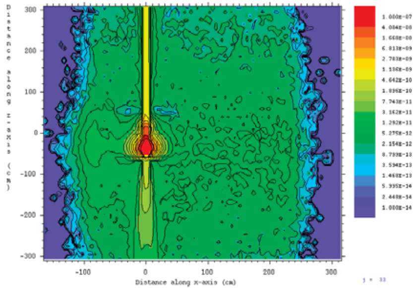
Figure 2.1.71: Photon dose rate contours in (\text{rem/h})/(\text{el/s}) in the xz -plane at y = 0 , (electron beam line), through the undulator protector. Electron beam enters from the bottom of the figure.
