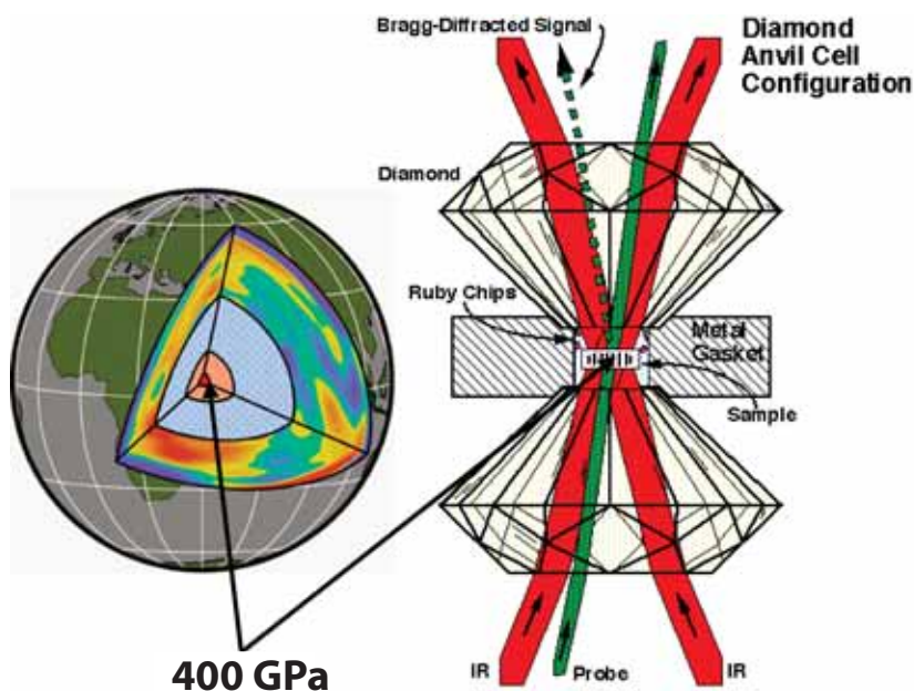
Figure 1.2.1: The Diamond Anvil Cell achieves center-of-the-earth pressures by squeezing specimens between small facets of two gem-quality diamonds.
