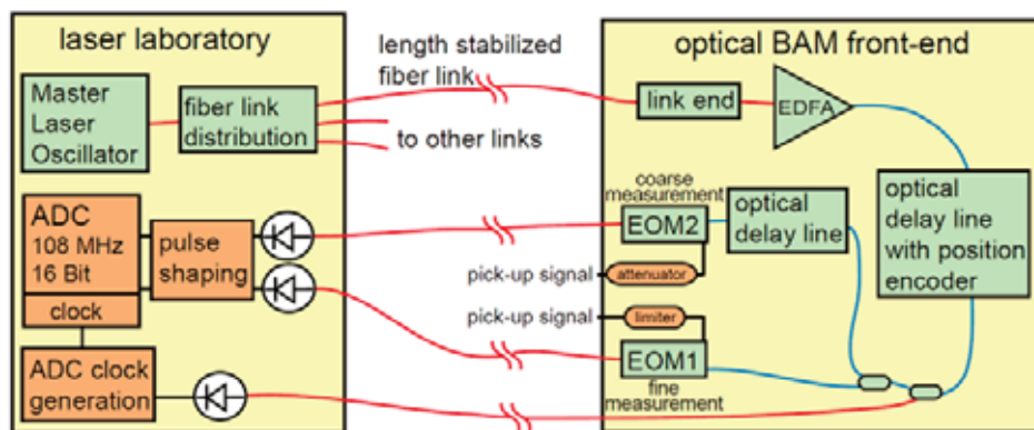
Figure 2.10.8: Schematic setup of the electro-optical detection scheme of the bunch arrival-time monitor (BAM) as it was used in first prototypes at FLASH (see [12]).
