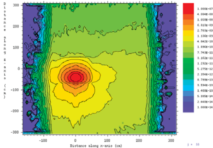
Figure 2.1.69: Neutron dose rate contours in (\text{rem/h})/(\text{el/s}) in the xz -plane at y = 0 , (electron beam line), through the undulator protector. Electron beam enters from the bottom of the figure.
