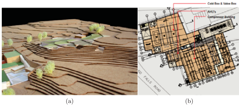
Figure 4.3.5: The cryoplant is recessed into the landscape as shown in the model image (a) on the left. The one-story, mainly underground building (b) houses the compressor room, an electrical substation, and the cold and valve boxes.
