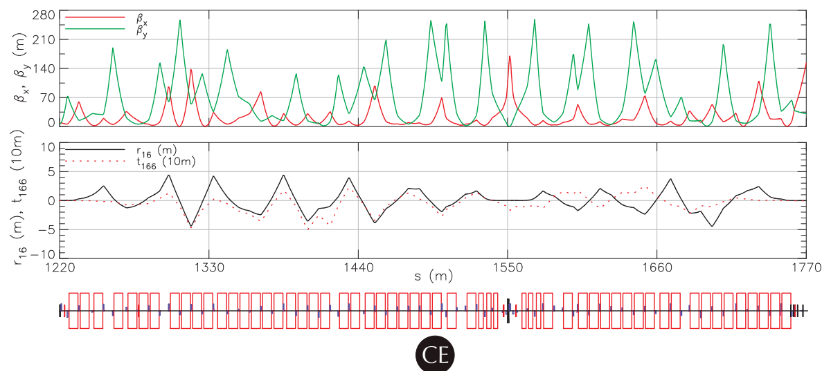
Figure 2.1.34: Optics for the CE section.
