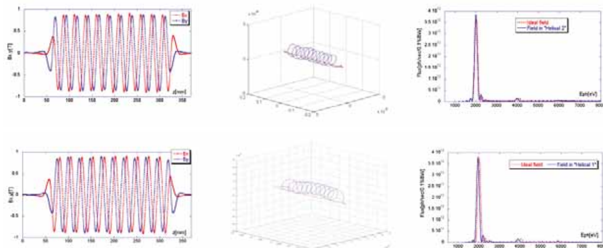
Figure 2.7.9: Left plots show vertical and horizontal field components measured in both helical modes corresponding to left and right x-ray polarizations. Central plots are 3D trajectories calculated for 5 GeV beam using measured magnetic field. Right plots are on-axis x-ray photon spectra calculated for measured and ideal fields.
