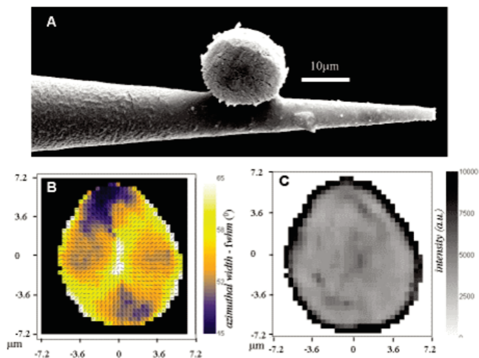
Figure 3.5.1: A: on-axis scanning electron microscopy image of laser-cut Kevlar-29 section glued to glass capillary, B: composite WAXS image of azimuthal width and radial texture based on a recursive analysis of the 200 reflection. The individual patterns were recorded with a 1\ \mu\text{m} beam. The skin zone shows more disorder; C: composite SAXS image of intensity of central scattering. The increased intensity in the skin-zone can be attributed to an oriented SAXS streak. An ERL soft matter beamline would allow studying skin-core structures on smaller fiber cross sections such as in electrospun fibers.
