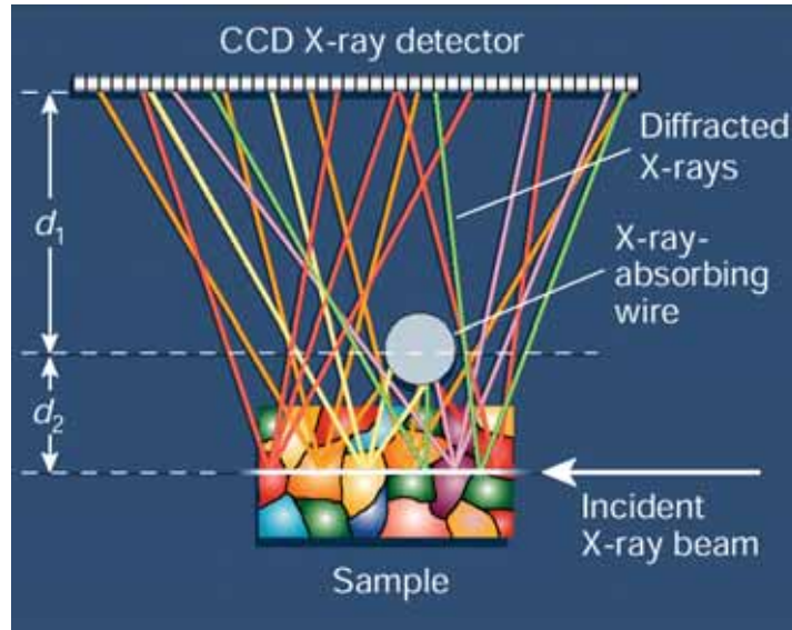
Figure 1.2.2: Differential-Aperture X-Ray Structural Microscopy (DAXM) from UniCAT beamline (APS). Schematic of the focusing geometry and depth profiling technique of DAXM. The x-ray diffraction patterns and analysis provide \approx 0.01^\circ angular resolution used to measure rotation gradients and subgrain structure within crystal grains [19].
