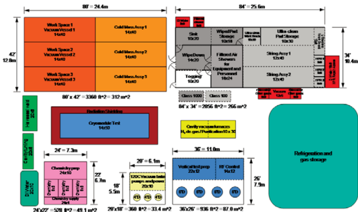
Figure 2.4.40: Block diagram of the space required for typical cryomodule production tasks to assemble two cryomodules per month.
