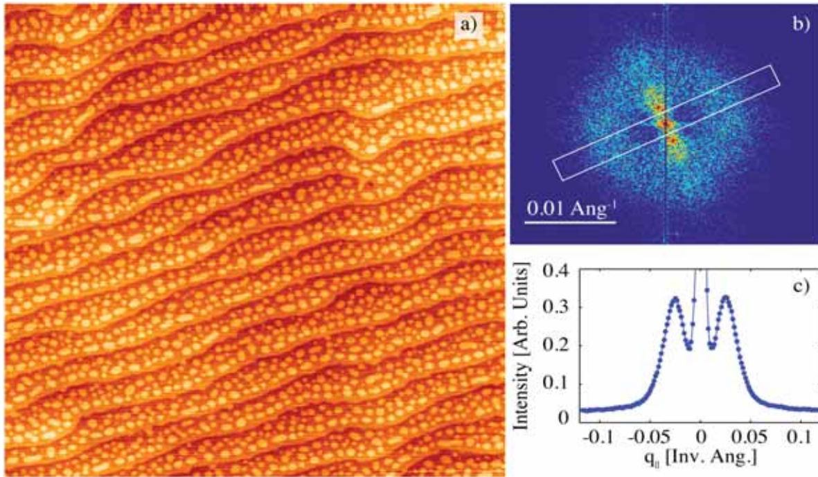
Figure 1.2.4: a) Atomic force microscope image of \langle 001 \rangle SrTiO 3 after pulsed-laser-deposition growth of 11.3 layers of SrTiO 3 . b) Fourier transformation of the AFM image, illustrating speckle in the diffuse ‘Henzler rings’ associated with the island structure. c) Diffuse scattering profile corresponding to the rectangular region in b, experimentally measured with an incoherent beam [44].
