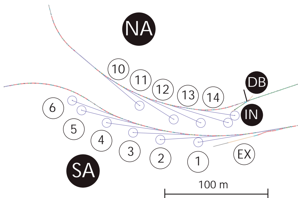
Figure 1.3.4: Layout for x-ray beamlines in the new user hall east of Wilson laboratory. Here IN is the injector, DB is the diagnostic beamline, NA is the north arc, and SA is the south arc. Numbers indicate x-ray beamlines. Beamlines 7–9 are in Wilson laboratory, G-line Annex, and G-line respectively. EX is the extracted beamline.
