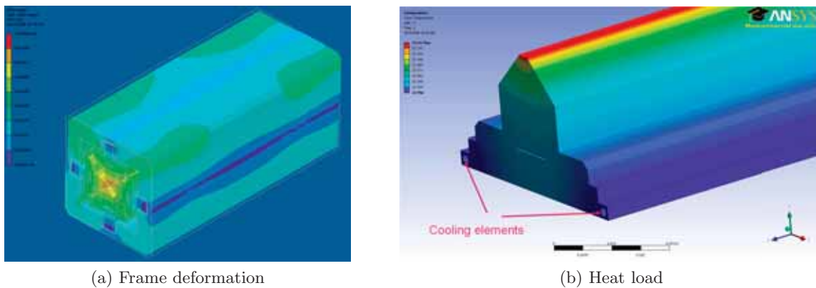
Figure 2.7.6: (a) Undulator frame deformation in the planar mode ranging from 3\ \mu\text{m} to 44\ \mu\text{m} , and (b) results of heat load analysis holding the device at 22^\circ\text{C} with a maximum increase of 0.16^\circ\text{C} .
