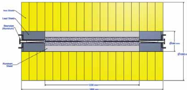
Figure 2.1.74: M type collimator. The top picture shows the overall collimator with iron shield (yellow),
