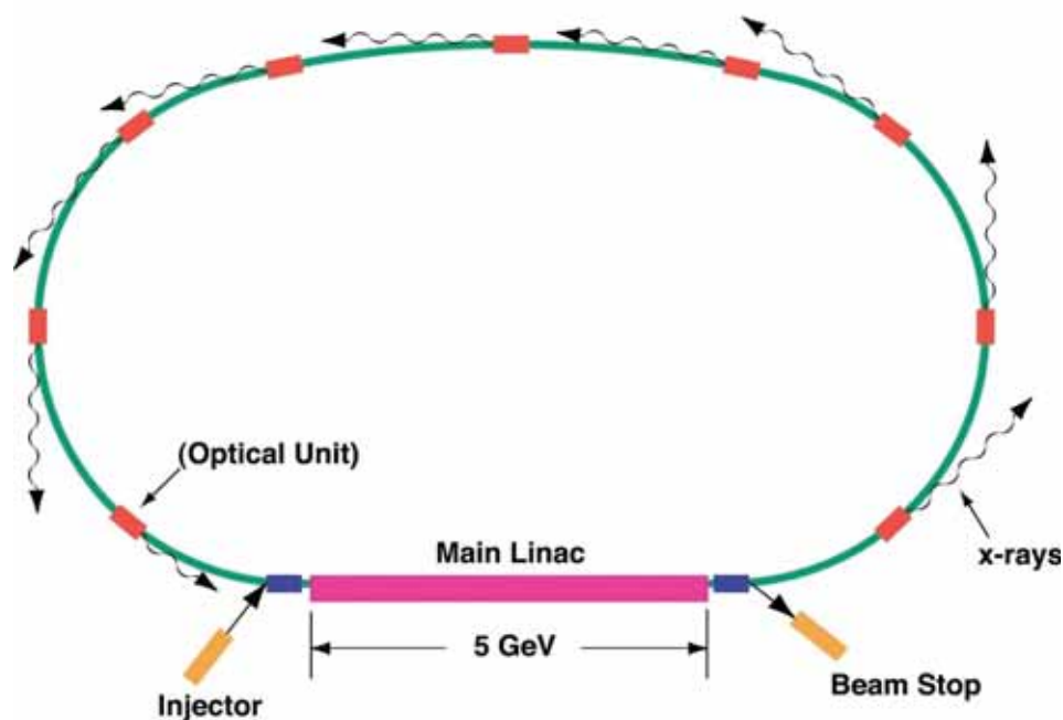
Figure 1.3.1: Schematic ERL facility consists (counterclockwise) of an electron injector, a superconducting Linac, beam stop, and transport-return loop-hosting undulators (red blocks) to generate beams of x-rays.
