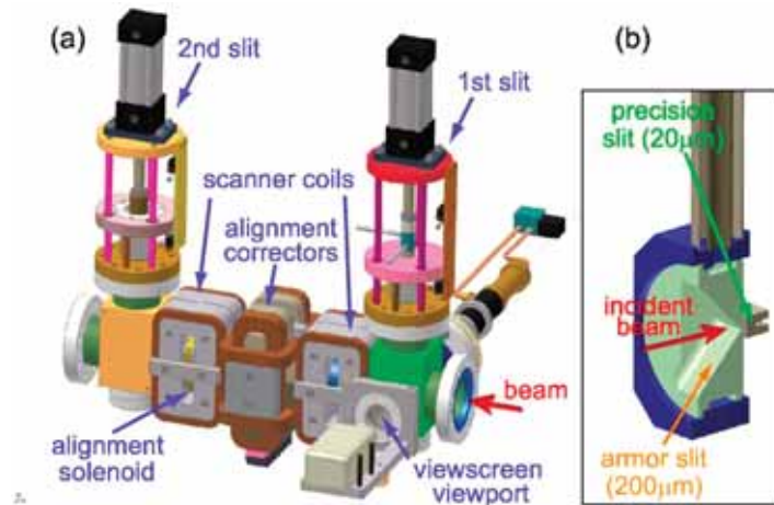
Figure 2.10.5: (a) Emittance measurement system as used downstream of the DC gun. The 15 MeV version of the device (not shown) is similar with the difference of a larger separation between the two slits (1.5 m). (b) details of one of the slits showing water cooled armor slit ( 80\ \mu\text{m} opening for the 15 MeV version) protecting the precision slit.
