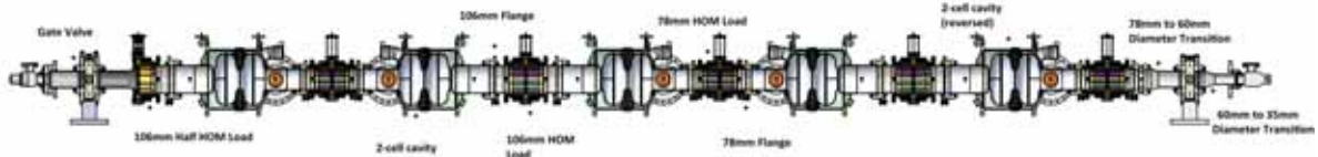
Figure 2.3.23: CAD model view of the Cornell ERL prototype injector cryomodule beam line with five 2-cell cavities. Note that the full ERL injector will have 12 2-cell cavities. Beam line components from left (beam entrance) to right (beam exit): gate valve; 106 mm half HOM load; first SRF cavity; 78 mm HOM load; second SRF cavity; 106 mm HOM load; third SRF cavity; 78 mm HOM load; fourth SRF cavity; 106 mm HOM load; fifth SRF cavity; 78 mm HOM load; 78 mm to 60 mm diameter transition; gate valve; 60 mm to 35 mm diameter transition.
