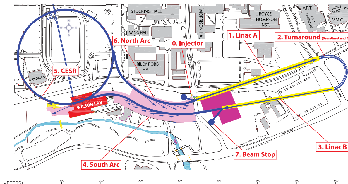
Figure 1.3.2: Schematic ERL layout incorporating the existing Cornell Electron Storage Ring (CESR). Electrons are injected (0) and accelerated to the right through a 2.7 GeV Linac (1), then looped through a turn-around arc (2), and accelerated to the left through an additional 2.3 GeV Linac (3) to 5 GeV. Beamlines are in the pink/red areas. Bunches then pass clock-wise around CESR (5). Bunches may be compressed to 100 fs (6) and feed more undulators before being uncompressed; their energy is recovered in second passes though Linacs (1) and (3). Finally they are stopped. Additionally a beam can be extracted after the second Linac (3) for bunch compression and novel radiation processes like the XFEL-O.
