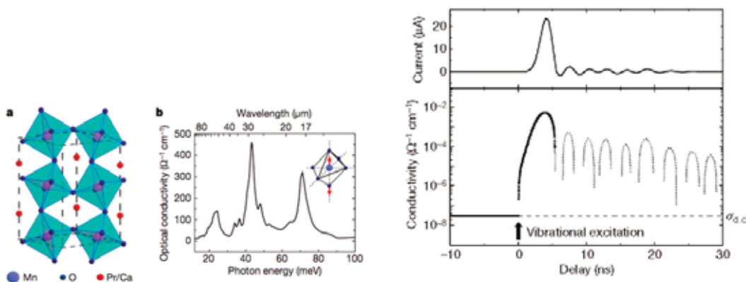
Figure 3.6.2: Time-dependent transport measurement. THz excitation ( 17.5\ \mu\text{m} , 1\ \mu\text{J}/\text{pulse} ) of the Mn-O stretching mode in \text{Pr}_{0.7}\text{Ca}_{0.3}\text{MnO}_3 results in a 10^3 increase in the sample current (upper panel) and a corresponding 10^5 increase in the sample conductivity (lower panel). The metastable metallic phase is both formed and relaxes within the experimental time resolution of 4 ns. From [6].
