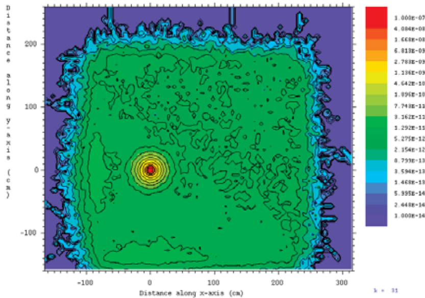
Figure 2.1.72: Photon dose rate contours in (\text{rem/h})/(\text{el/s}) in the xy -plane at z = 0 through the undulator protector.
