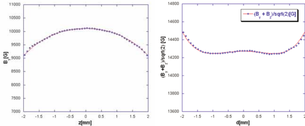
Figure 2.7.4: Field roll-off in helical (left) and planar (right) modes.
