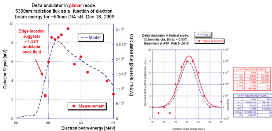
Figure 2.7.12: Radiation intensity measured at 5300 nm as a function of electron beam energy (left plot) with the Delta undulator in the planar mode. Radiation intensity at 4500 nm wavelength (right plot) as a function of electron beam energy for the Delta undulator model in the helical mode.
