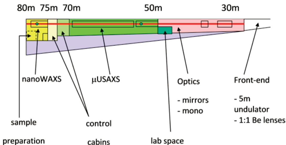
Figure 3.5.2: Possible layout for a microbeam scattering beamline.
