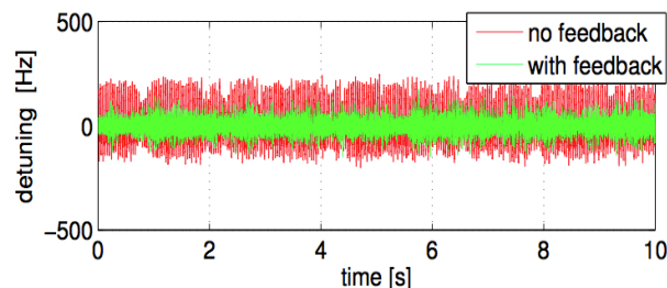
Figure 9: Microphonics compensation by a fast piezoelectric tuner in feedback mode.
