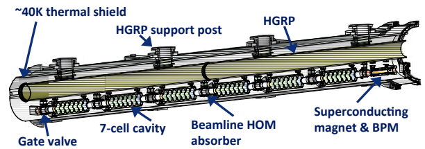
Figure 4: Cross-section of the ERL main linac module with six SRF cavities and HOM beamline absorbers in between.
