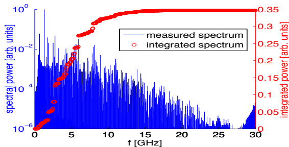
Figure 3: HOM spectrum excited by the beam as measured at one of the HOM loads. The integrated spectrum is plotted on the secondary axis.
