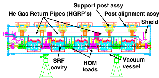
Figure 1: Cross-section of the ERL injector module with 5 SRF cavities and HOM beamline absorbers in between.
