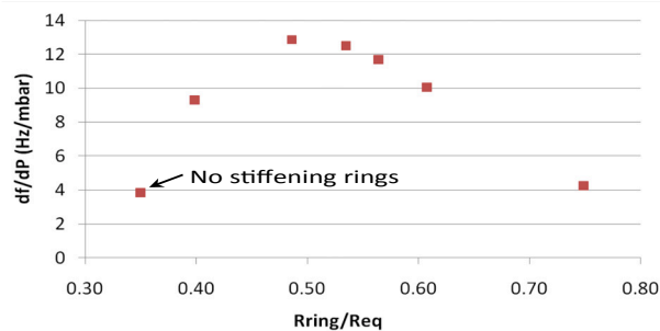
Figure 7: Sensitivity of the fundamental mode frequency to small changes in the LHe bath pressure vs. radius of the stiffening rings between the cells (ANSYS simulations).
