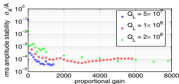
Figure 8: Measured RF field amplitude stability vs. proportional gain for a 9-cell cavity operated at different loaded quality factors in presence of \approx 30 Hz peak microphonics.
