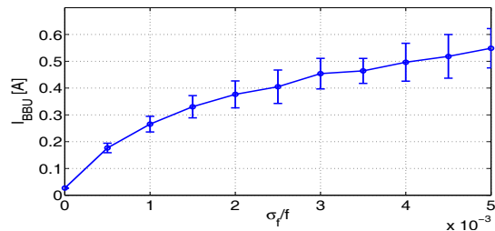
Figure 6: Simulated BBU current in the Cornell ERL main linac vs. relative HOM cavity to cavity frequency spread.
