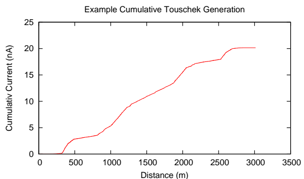
Figure 3: Integral over Touschek particle generation for CERN lattice version 3.0. \epsilon_{n,x,y} = 3.0 \times 10^{-7} m. Bunch charge is 77 nC and repetition rate is 1.3 GHz.
