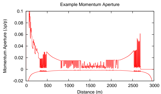
Figure 2: Example momentum aperture from CERN lattice version 3.0. The positive aperture is determined entirely by beam pipe collisions. The negative aperture is dominated by stopping during deceleration.
