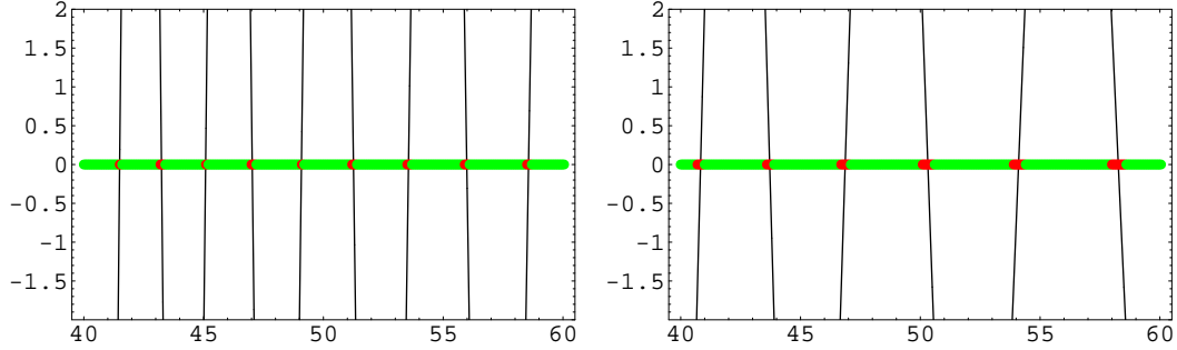
Fig. 2. Trace of the ion oscillation matrix for different \beta_y(\text{m}) for \text{CH}_4^+ (left) and \text{CO}_2^+ (right).
