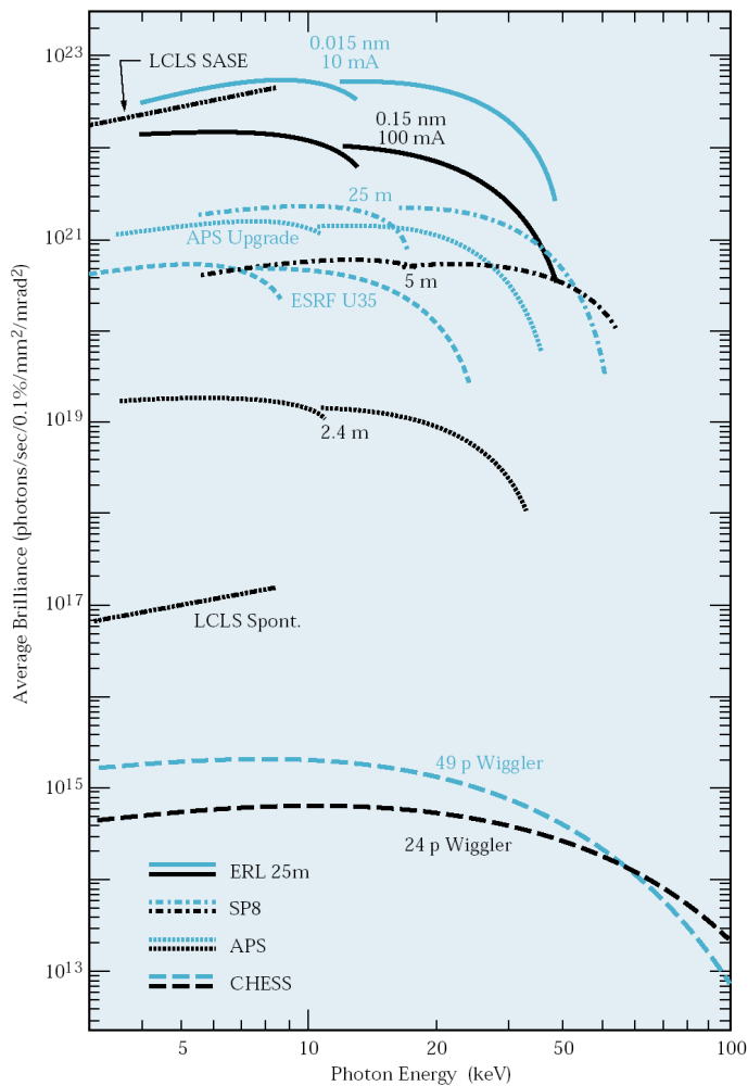
Fig. 2a Expected ERL average brilliance vs. x-ray energy in the high-flux (100 mA) mode as compared with the CHESS, ESRF, APS, and Spring-8 storage ring sources and the LCLS in SASE mode.
