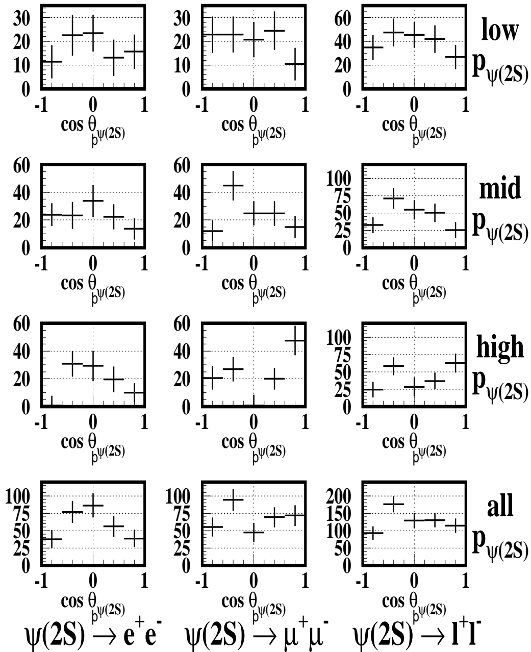
Figure 5.7: Data: \psi(2S) decaying via \psi(2S) \rightarrow \ell^+ \ell^- .
