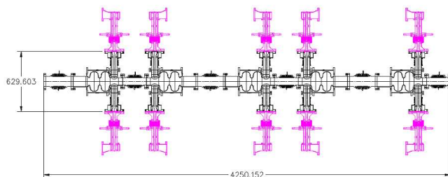
Figure 1: Cavity layout for Cornell ERL prototype injector.
