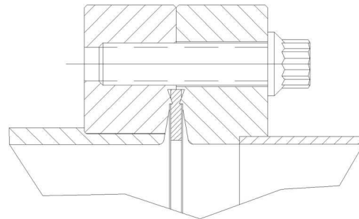
Figure 5: New design of the Conflat flange for the 2-cell injector cavity.
