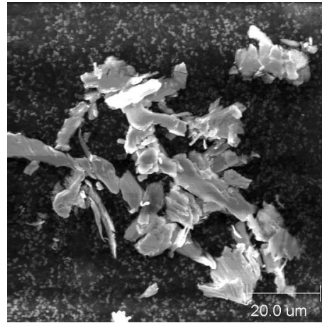
Figure 4: Copper particles generated from RF fingers.
