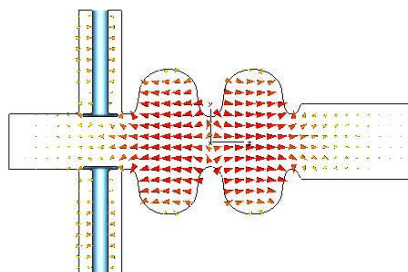
Figure 2: 2-cell cavity with twin RF input couplers.
