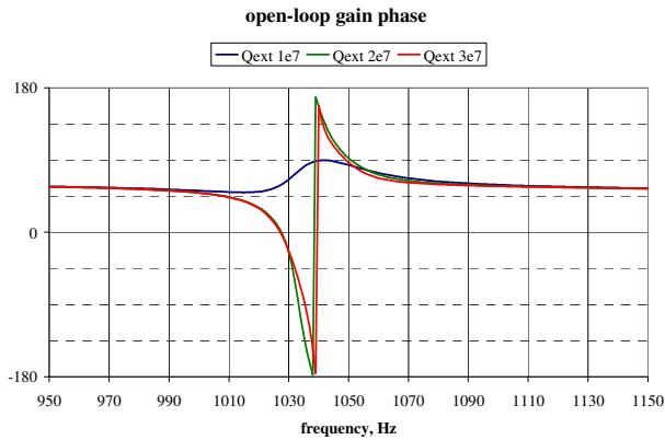
Figure 4: Open-loop Bode plot for different values of passive cavity quality factor (50 mA beam current).
