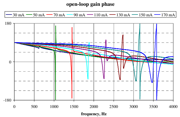
Figure 5: Open-loop Bode plot for different beam currents and the passive cavity parameters Q_{\text{ext}} = 2 \times 10^7 , V = 1.2 MV.
