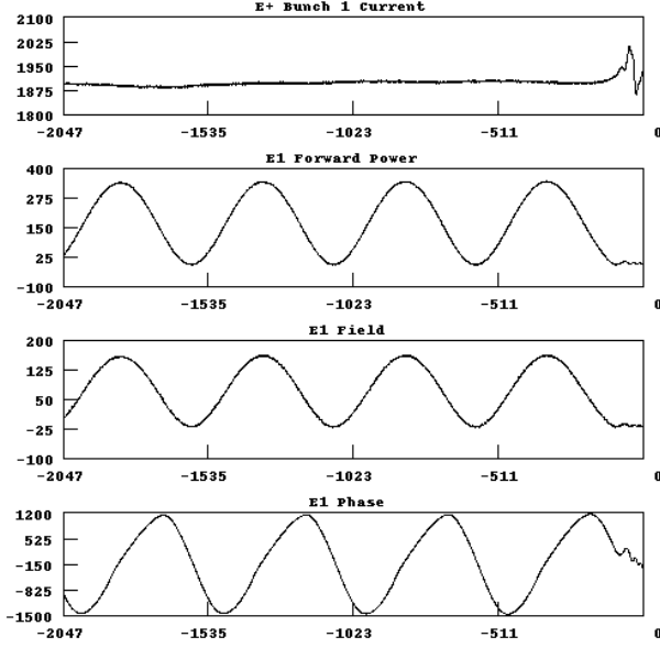
Figure 1: Beam loss plots of the passive cavity signals. Vertical axes are in arbitrary units, horizontal axis is the number of revolution periods (1 period = 2.56 \mu s). The “E1 forward power” signal represents the forward wave power in the resonant waveguide.
