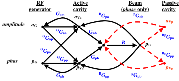
Figure 2: Signal-flow graph of the RF system.
