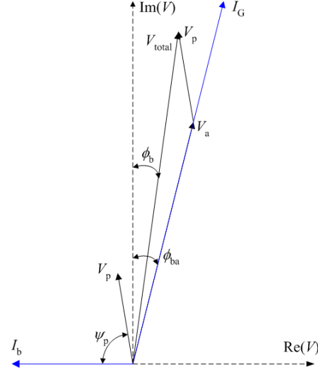
Figure 3: Phasor diagram.
