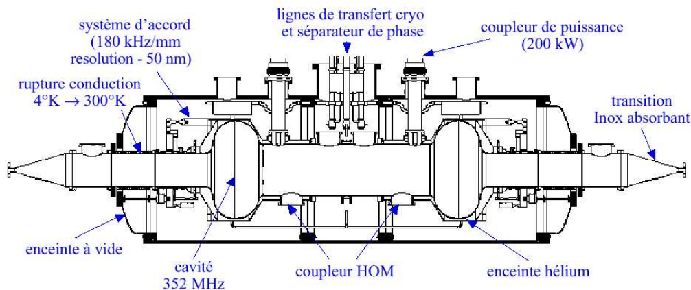
Figure 6: SOLEIL cryomodule [30].
