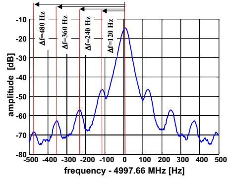
Figure 3: Spectrum of the 500 MHz CESR reference signal before improvements have been made.
