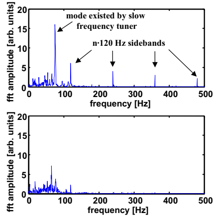
Figure 2: Measured microphonics spectrum. Top: Fourier transform of the cavity detuning signal shown in Figure 1 (before improvements have been made). Bottom: Fourier transform of the cavity detuning signal shown in Figure 4 (after improvements have been made).
