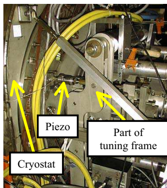
Figure 5: CESR cryostat with piezo frequency tuner.
