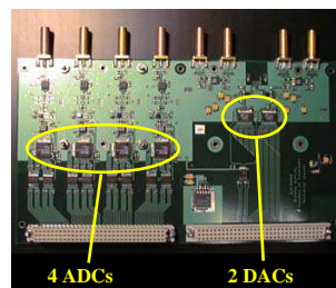
Figure 3: ADC/DAC daughter board.
