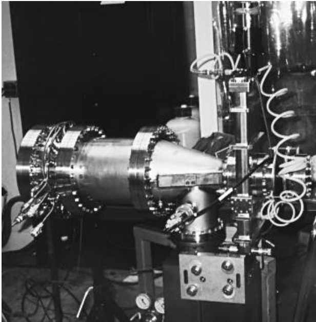
Figure: 4 Beam line assembly: HOM load, taper, gate valve and sliding joint.
