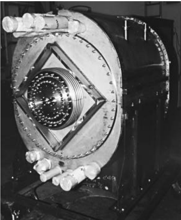
Figure: 2 MARK II cryostat: fluted beam tube end.
