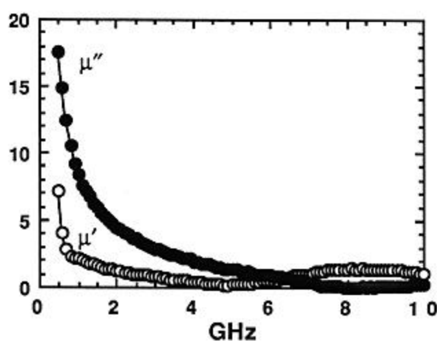
Figure 2. Measured values of \mu_r for Ferrite-50.
