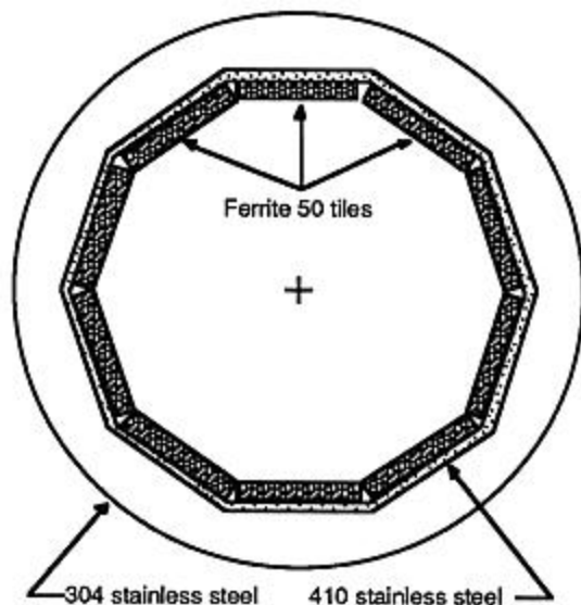
Figure 4. Ferrite beam tube load concept.
