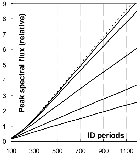
Figure 2: Undulator peak spectral flux vs number of periods improves significantly with reduced electron energy spread. Solid curves are based on the formula and assumptions in the text. They correspond to \delta\gamma/\gamma = 0.15\% (lowest curve), 0.1% (typical 3 rd generation value), 0.05, 0.02 (proposed ERL), and 0.01%. For the dashed curve \delta\gamma/\gamma = 0 so the finite electron emittance limits peak flux. See [12] for additional machine parameters.
