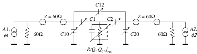
Figure 6: Equivalent diagram.
