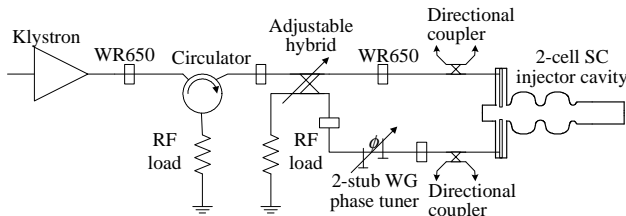
Figure 1: RF power splitting scheme for ERL injector.
