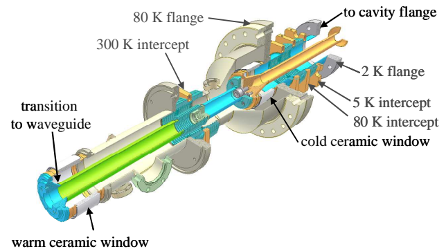
Figure 2: 3D view of the injector cavity coupler.
