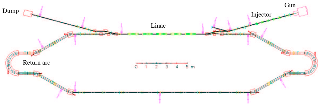
Figure 1: Layout of the Cornell ERL Prototype
