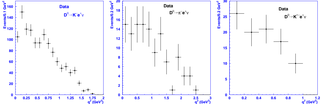
FIG. 11: Uncorrected q^2 distributions for D^0 \rightarrow K^- e^+ \nu , D^0 \rightarrow \pi^- e^+ \nu , D^0 \rightarrow K^{*-} e^+ \nu .
