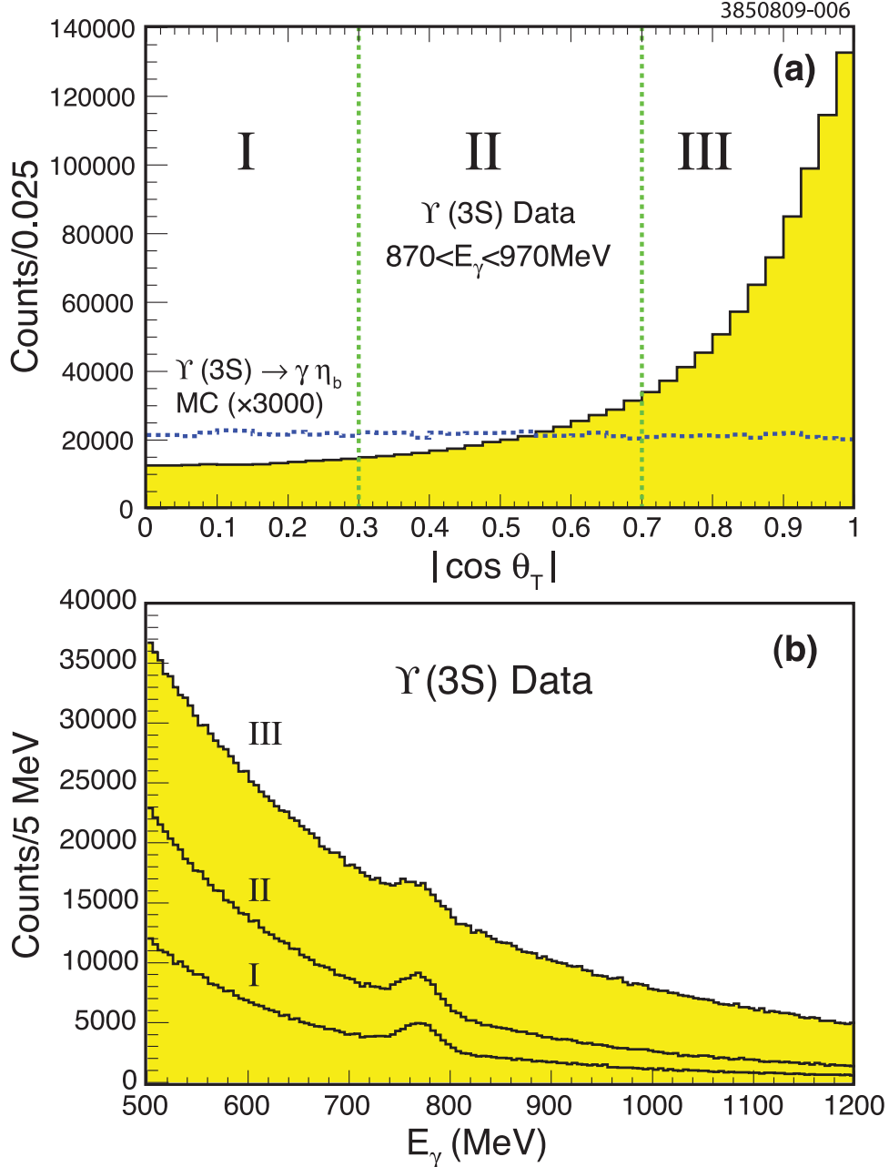
FIG. 1: (a) Distribution of |\cos \theta_T| for \eta_b signal MC events (dotted) and background dominated \Upsilon(3S) data (shaded) in three regions, I, II, and III defined in the text. (b) The E_\gamma distribution from \Upsilon(3S) data in the three regions of |\cos \theta_T| . Only the \chi_{bJ}(2P) \rightarrow \gamma \Upsilon(1S) lines at around 770 MeV are visible above the background.
