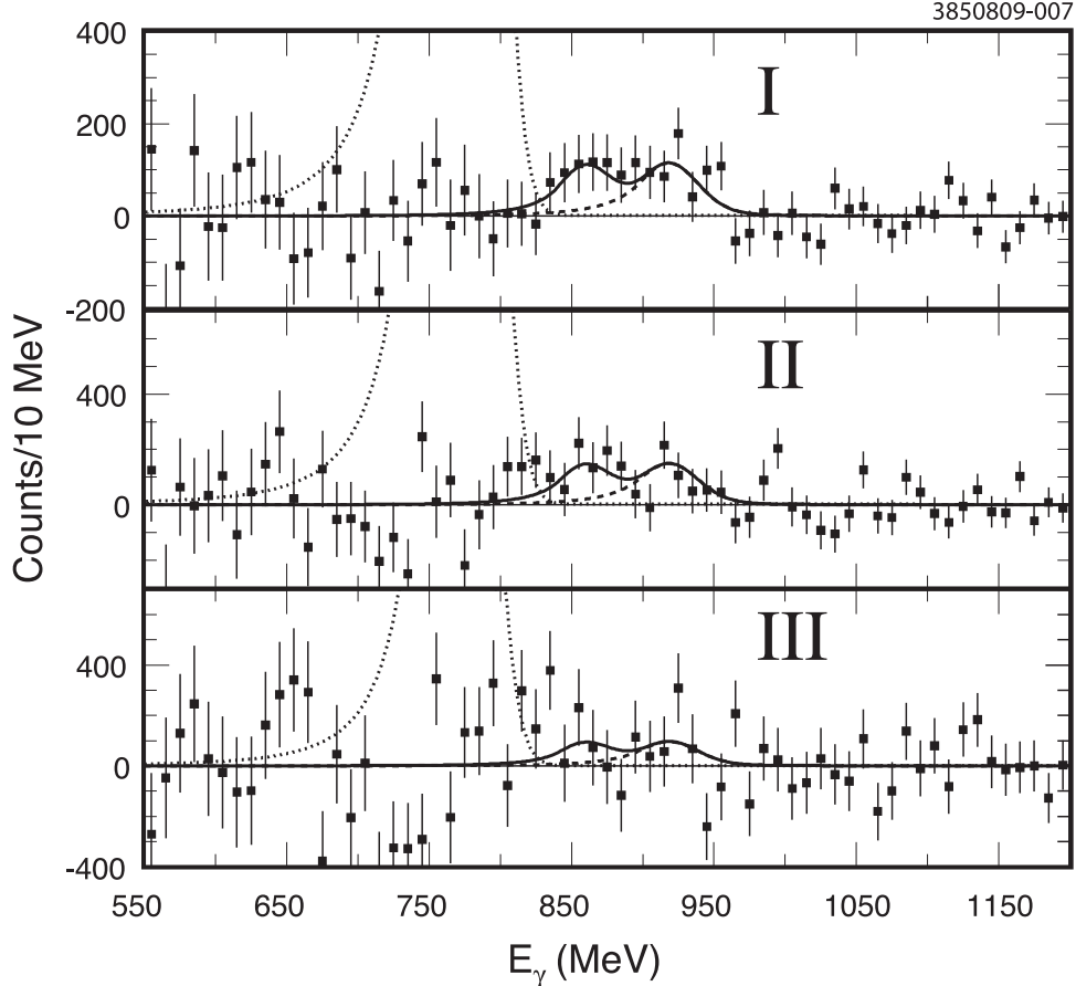
FIG. 2: Background and \chi_{bJ}(2P) subtracted distributions of E_\gamma from \Upsilon(3S) decays in three |\cos\theta_T| regions, I, II, and III defined in the text. The curves are the joint fit results. The \chi_{bJ}(2P) peaks are indicated by the dotted lines and the \eta_b signals by the dashed lines, which join the solid line.
