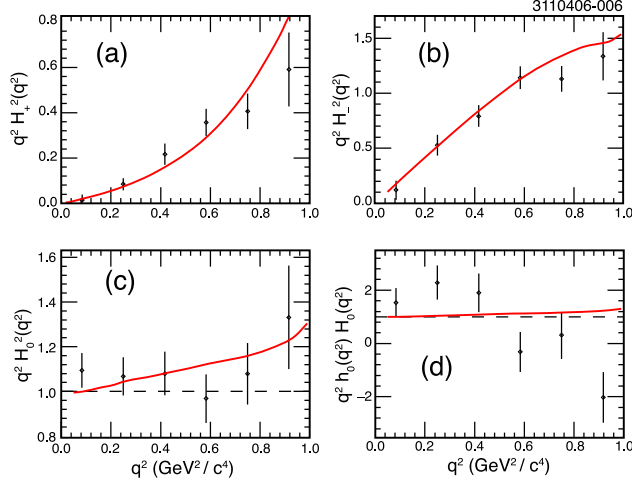
FIG. 5: Measured form factor products for six q^2 bins. The data are points with error bars representing only the statistical uncertainties. The solid curves are obtained using the form factor representation and the parameters reported in Ref. [7], namely: V(0)/A_1(0) = 1.505 , A_2(0)/A_1(0) = 0.875 , and s -wave parameters \mathcal{A} = 0.33 and \delta = 39^\circ . The histogram plots are: (a) q^2 H_+^2(q^2) , (b) q^2 H_-^2(q^2) , (c) q^2 H_0^2(q^2) , and (d) q^2 h_0(q^2) H_0(q^2) .
