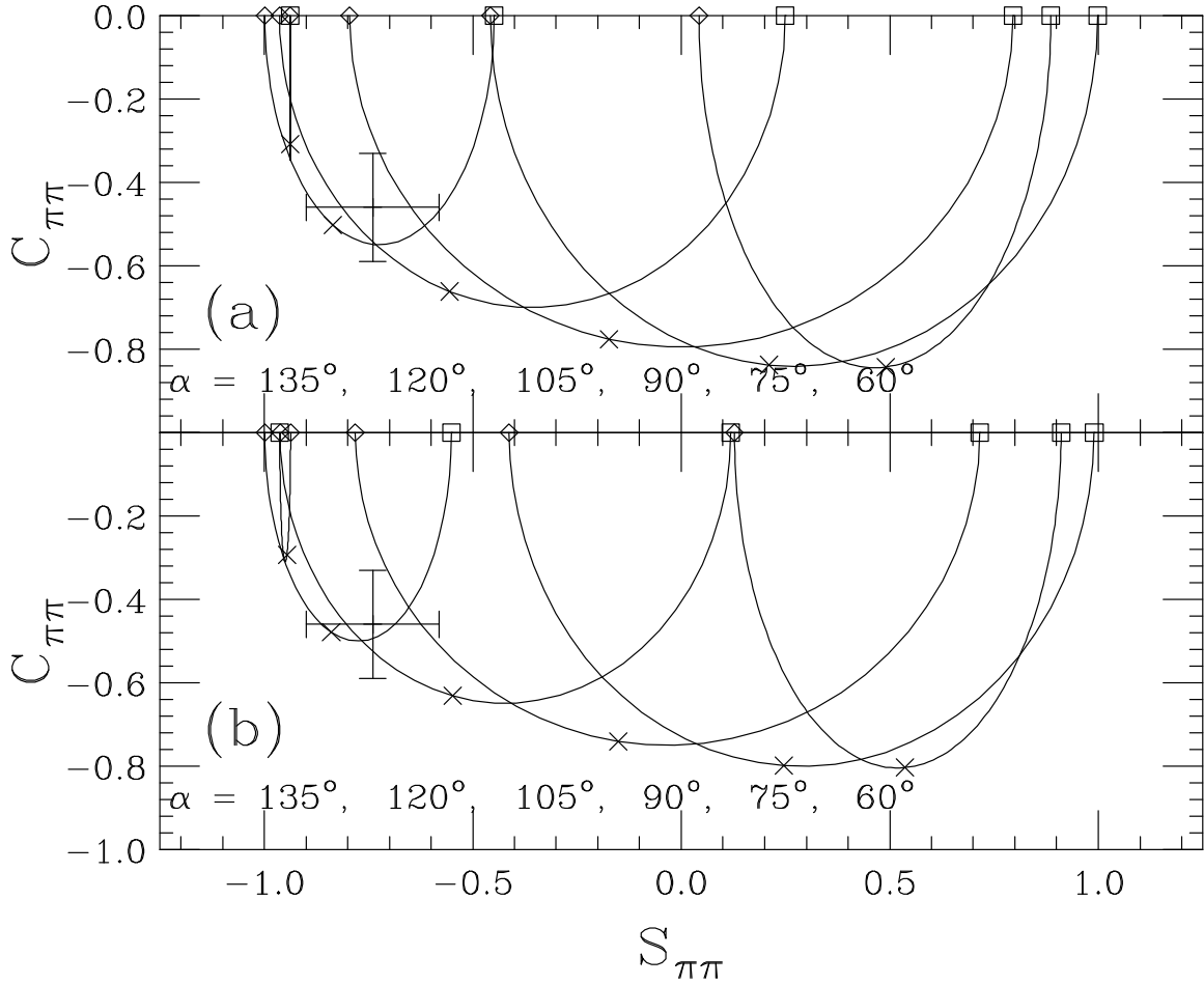
Figure 1: Parametric curves of C_{\pi\pi} vs. S_{\pi\pi} for the range -\pi \leq \delta \leq 0 , based on measurements of (a) \mathcal{R}_+ and (b) \mathcal{R}_0 . Points marked with diamonds, crosses and squares denote \delta = 0 , -\pi/2 and -\pi , respectively. Plotted point denotes the experimental average (3).
