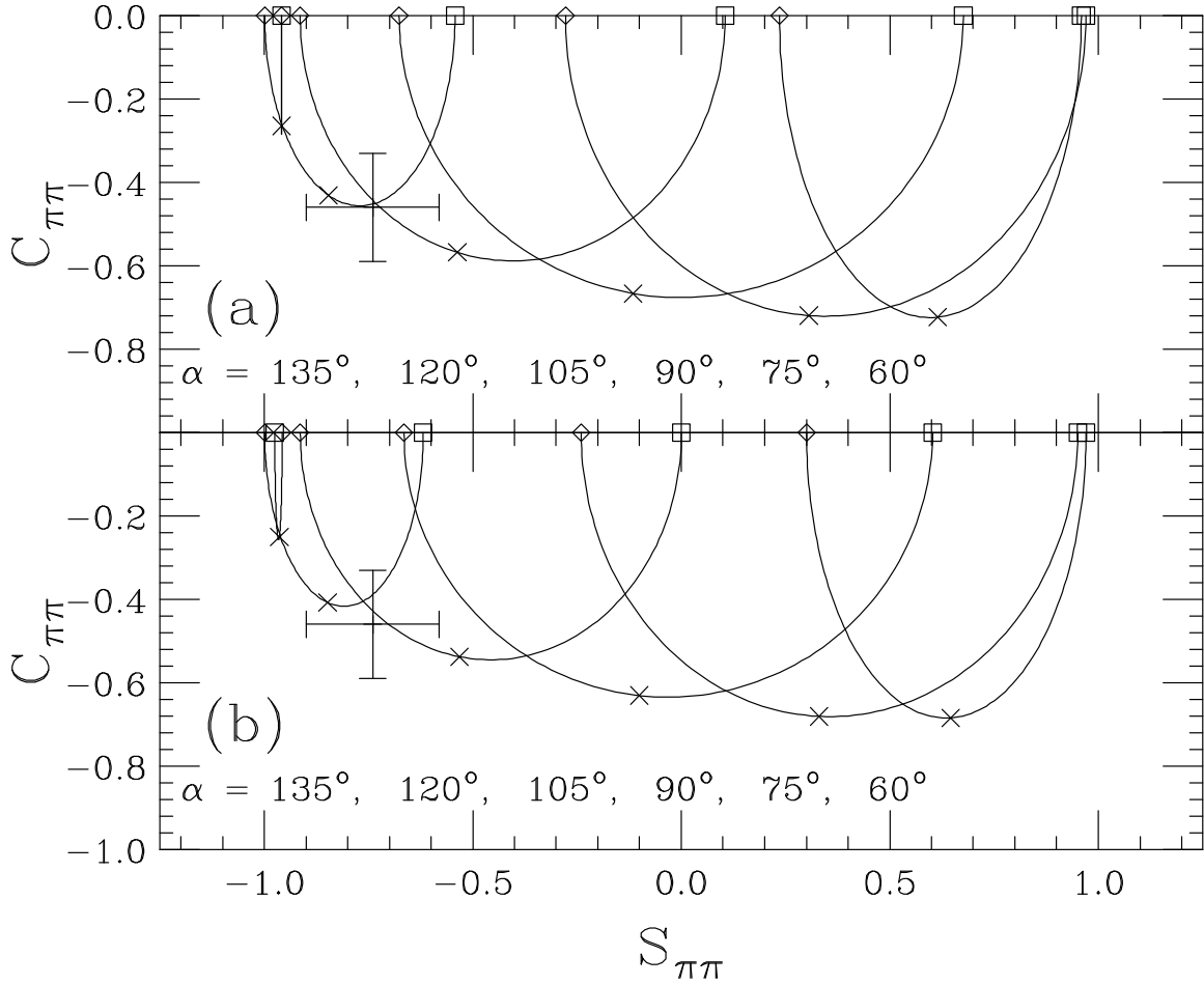
Figure 2: Same as Figs. 1 but with SU(3) breaking included in penguin terms as explained in text.
