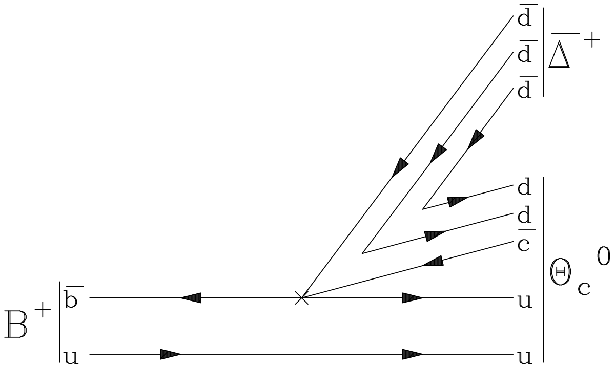
Figure 6: Production of a charmed exotic baryon \Theta_c^0 = uudd\bar{c} in B^+ decays.
