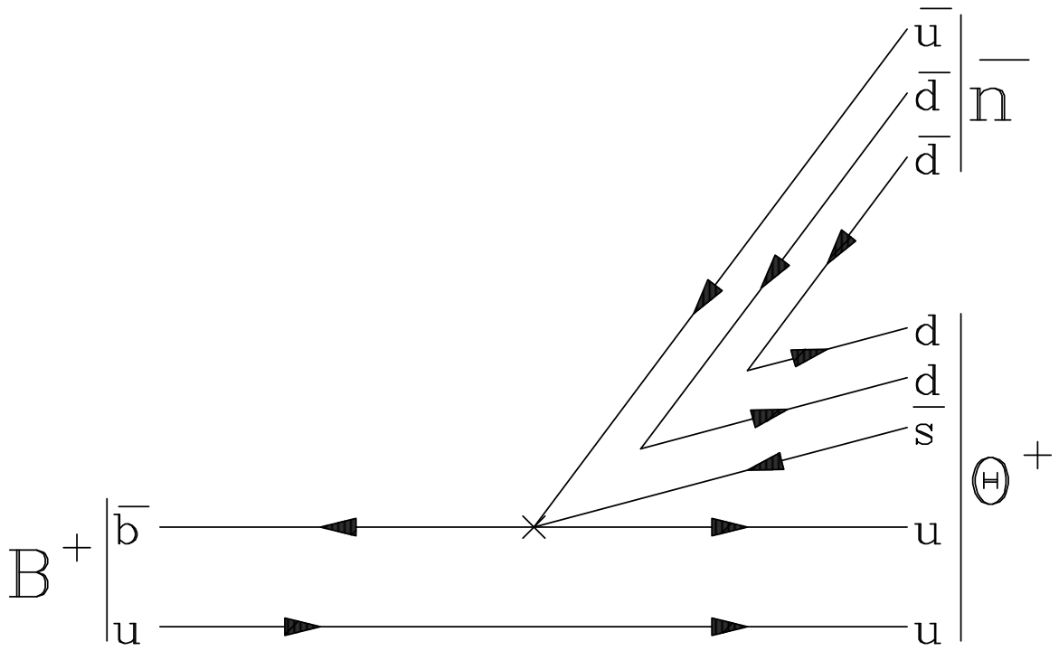
Figure 7: Production of an exotic baryon \Theta^+ = uudd\bar{s} in B^+ decays.
