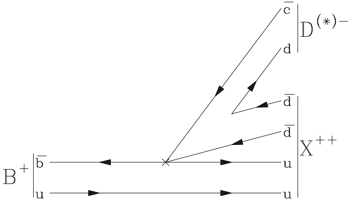
Figure 2: Production of an exotic meson X^{++} = uu\bar{d}\bar{d} in B^+ decays. If the recoiling charmed meson is a D^{*-} , identification may be easier through the decay D^{*-} \rightarrow \pi^- \bar{D}^0 .
