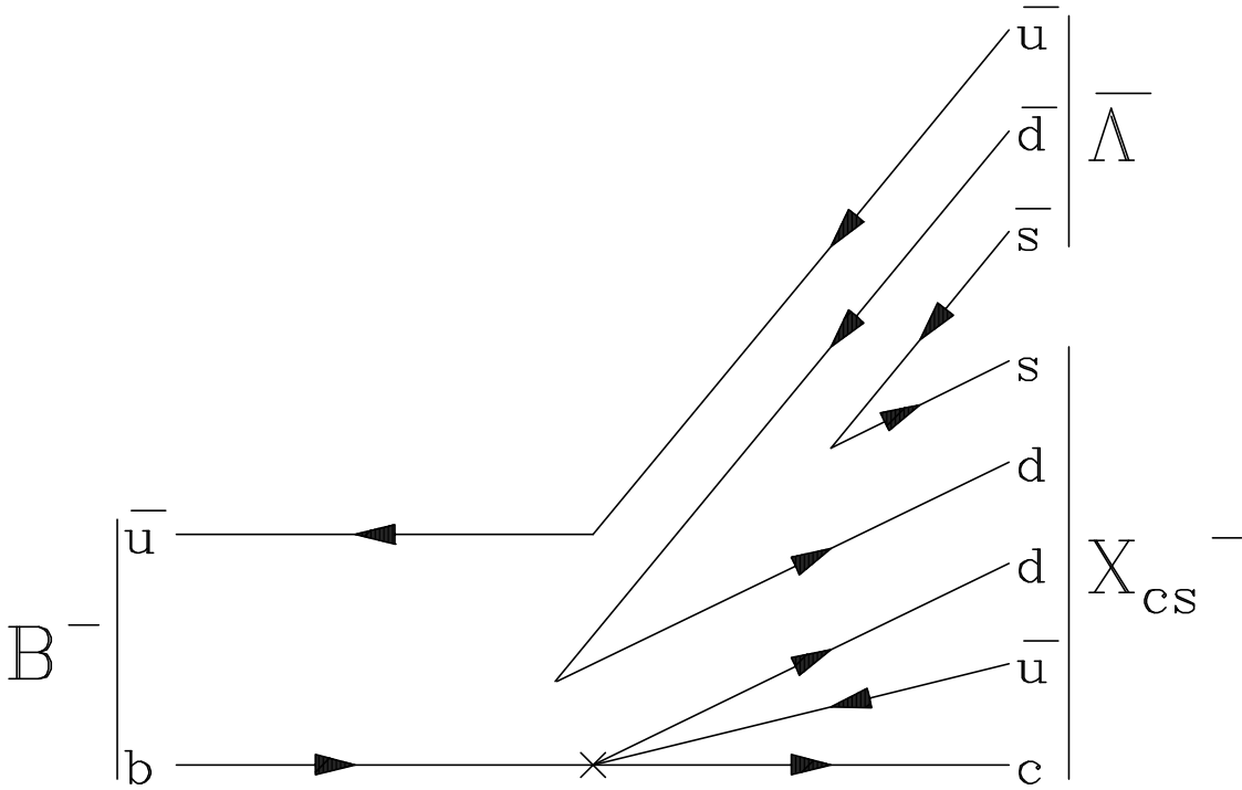
Figure 5: Production of a charmed-strange exotic baryon X_{cs}^- = cdds\bar{u} in B^- decays.
