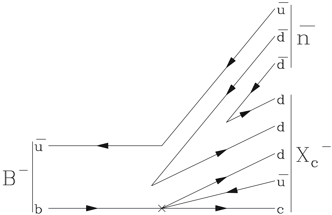
Figure 4: Production of a charmed exotic baryon X_c^- = cddd\bar{u} in B^- decays.
