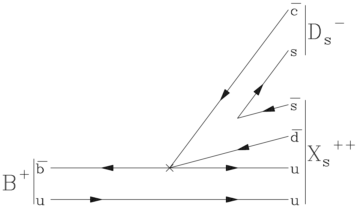
Figure 3: Production of a strange exotic meson X^{++} = uu\bar{d}\bar{s} in B^+ decays.
