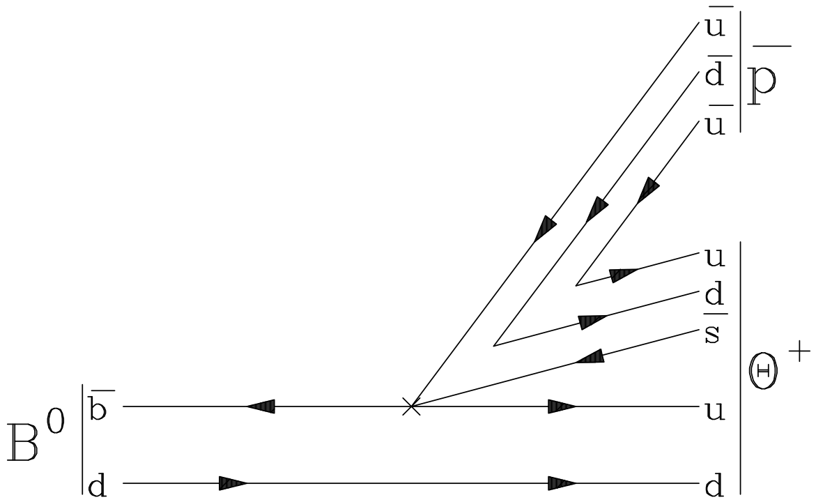
Figure 8: Production of an exotic baryon \Theta^+ = uudd\bar{s} in B^0 decays.
