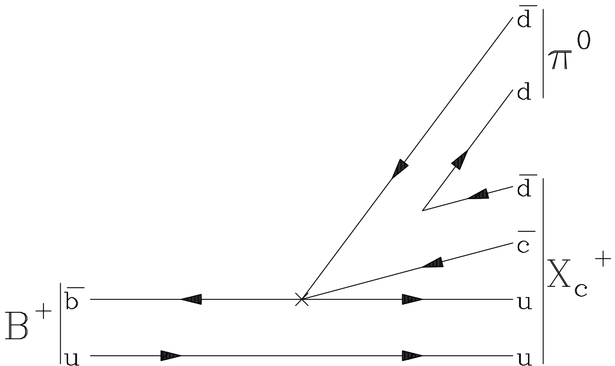
Figure 1: Production of an exotic meson X_c^+ = uu\bar{c}\bar{d} in B^+ decays. The \pi^0 could also be a photon or any other neutral particle. Here and subsequently the weak vertex is denoted by \times .
