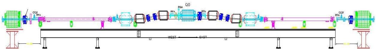
Figure 5: Beam chicane setup at North area with new-made undulators. The same setup could be used in L0, South Area; previous Figure.
