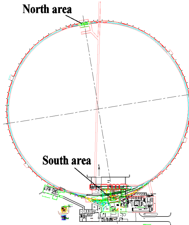
Figure 3: Possible locations for equipment at CESR. Location at the North area is preferable.
