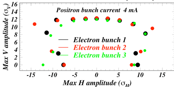
Figure. 5. Dynamic aperture with BBI compensation.
