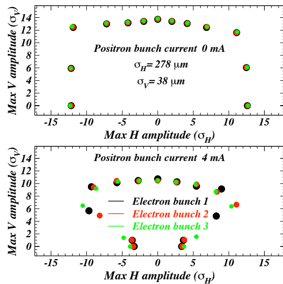
Figure. 4. Modeled dynamic aperture for the design optics. Units are horizontal \sigma and fully coupled vertical \sigma at the IP.
