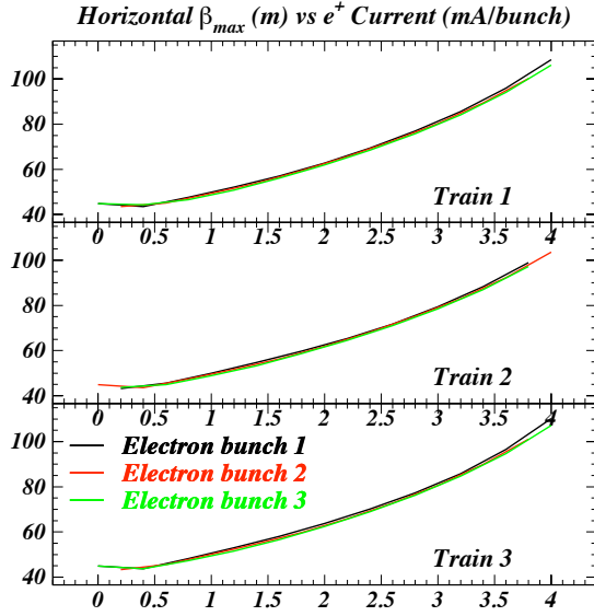
Figure. 2. Maximum horizontal \beta -functions for 3 trains. measured and found to be in good agreement with the model calculation[3].
