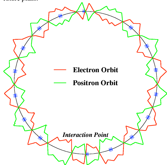
Figure. 1. Closed orbits for electrons and positrons
