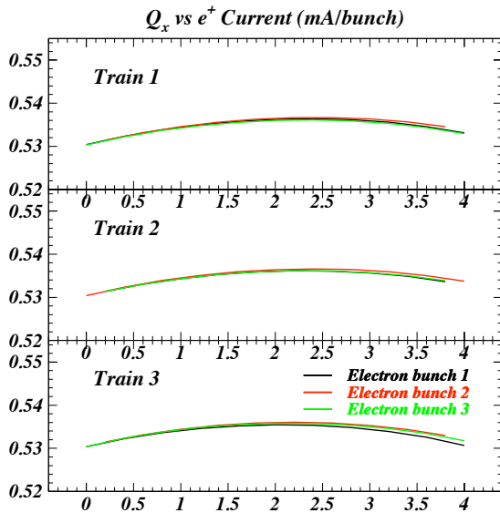
Figure. 3. Horizontal tunes for different trains.
