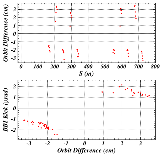
Figure 3: Modeled orbit separation and resulting BBI kicks in the 5x5 configuration employed to measure the orbit distortions shown in Fig. 4
