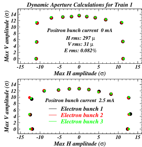
Figure 6: Comparison of the electron dynamic aperture in the distortion-free optics (upper plot) to that in the optics distorted by 2.5 mA/bunch in the positron beam (lower plot). The aperture is calculated at the interaction point in units of RMS beam size. The vertical beam size is the value assuming full coupling. The lattice design procedure developed to account for the effects of the parasitic crossings yields an improved aperture at the operating current.
