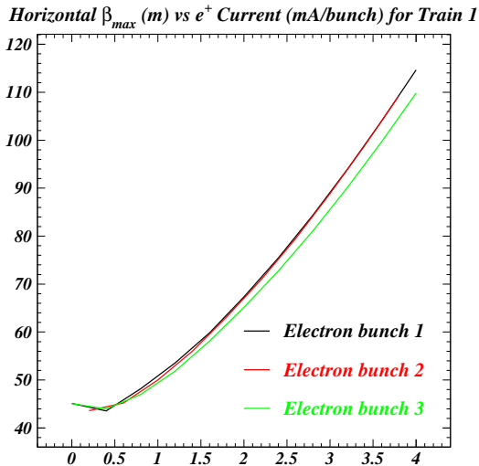
Figure 5: Maximum value of the electron horizontal beta function the CESR-c optics as a function of the positron bunch current
