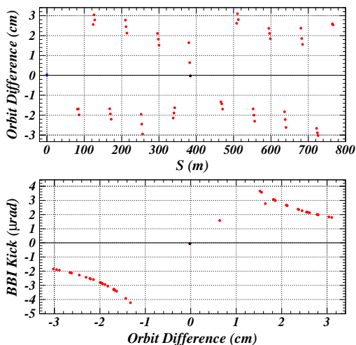
Figure 2: Horizontal positron-electron orbit difference at the crossing points in the CESR-c model of the operational 8x3 configuration as a function of their position around the ring (upper plot) and the horizontal kicks resulting in the Bassetti-Erskine approximation as a function of this orbit difference (lower plot). The black point indicates the crossing diametrically opposed from the main interaction point, where the separation is vertical.
