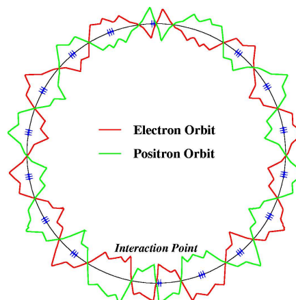
Figure 1: Electrostatic separators establish closed-orbit waves separating the electron and positron beams at the positions of the parasitic crossings (blue lines), shown here for the particular case of the first bunch of the first electron train against the counter-rotating positron configuration of three bunches in each of eight trains. This is the present operational configuration for CESR-c.
