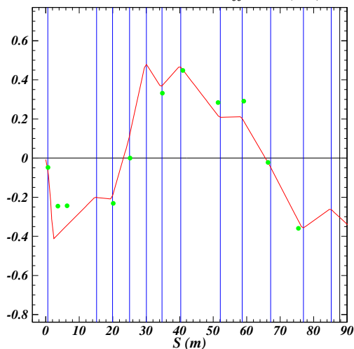
Horizontal Electron Orbit Difference (mm)
