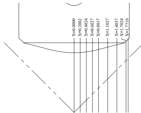
Figure 4: Lamination hyperbolic/flat pole-tip profile shape reference check points shown in inches.
