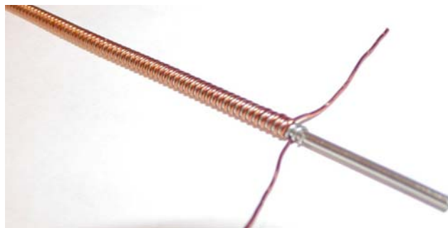
FIGURE 2: Central core first try. The winding done with pair of SC wires and pair of iron ones at once. Period of the winding is 2.42 mm. StSt tube has diameter 1.5 mm.
