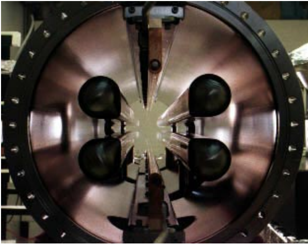
Figure 2: The electrode structure of the CESR separators.
