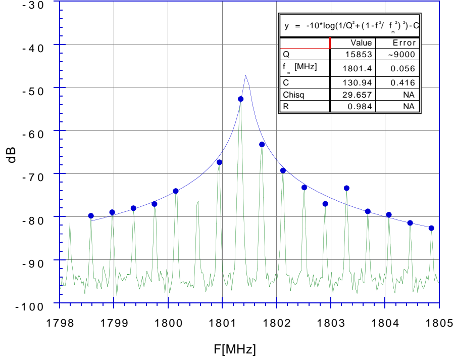
Resonance fitting of the measured single bunch spectra around 1800 MHz. East RF cavity 1, cell 4.
