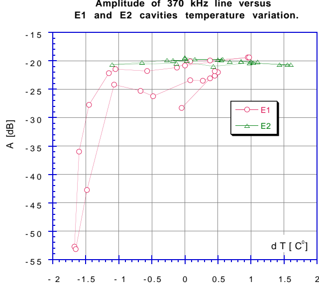
Figure 1: Amplitude of 370kHz line versus East RF cavities temperature.
