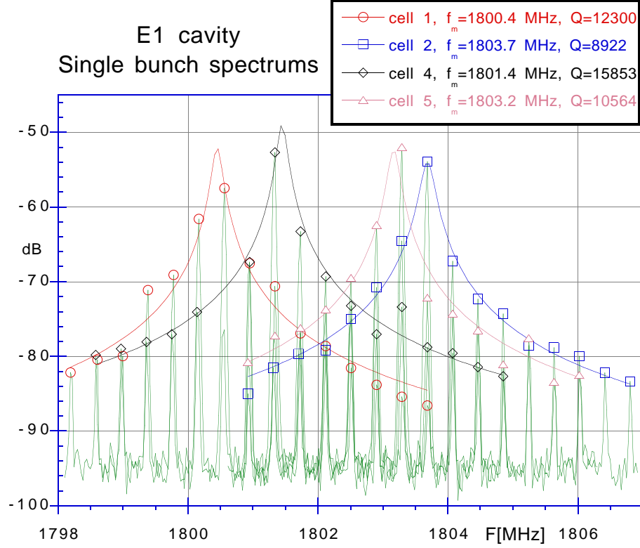
Figure 7: Spectra of the signals from four cells of the E1 cavity showing TM0-Mx-3 mode excitation
