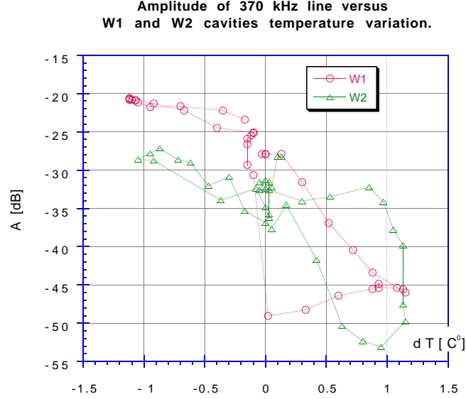
Figure 2: Amplitude of 370kHz line versus West RF cavities temperature.
