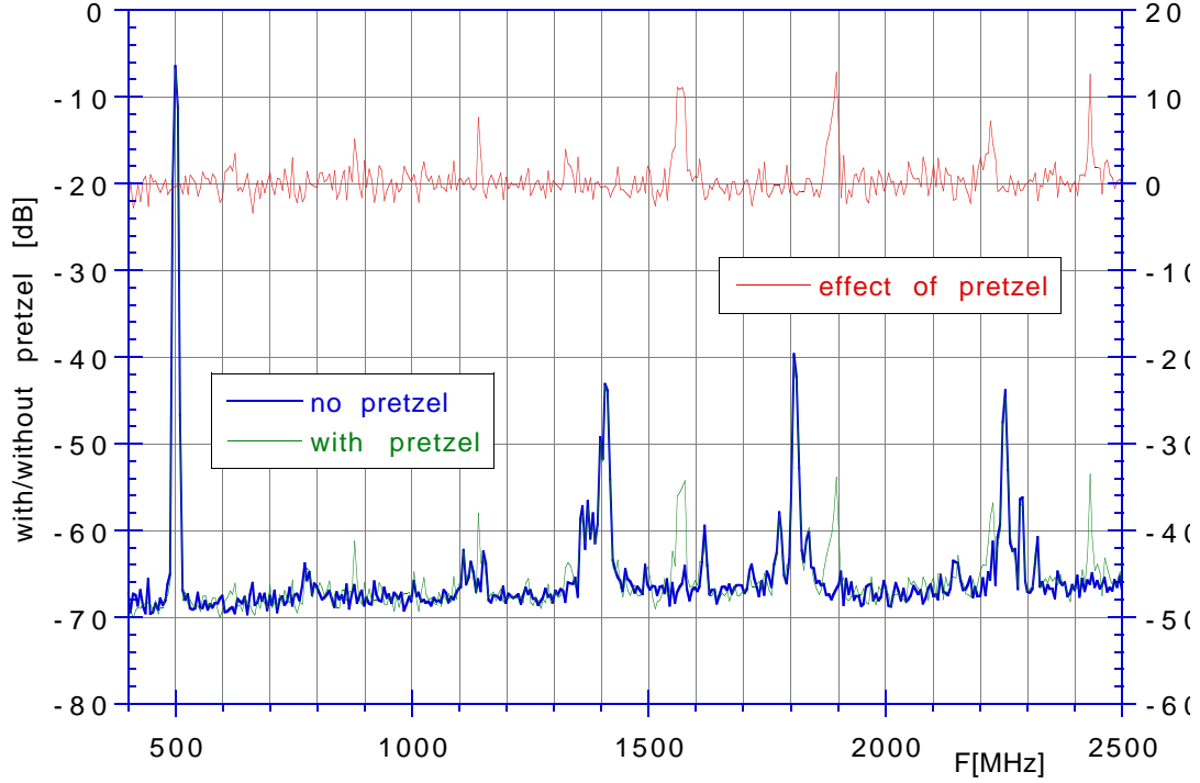
Figure 3: Spectra of signal from field probe of E1 cavity cell 4.
