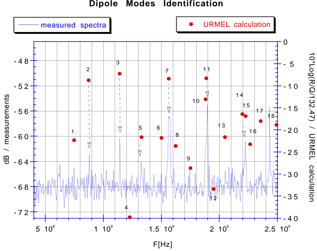
Figure 5: Dipol modes identification.
