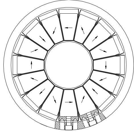
Figure 1: Phase-III Permanent Magnet Cross-section view.
