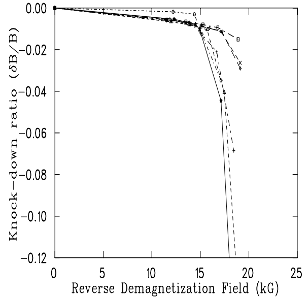
Figure 2: Knock-down ratio vs the applied external reversal field for several magnet pieces.
